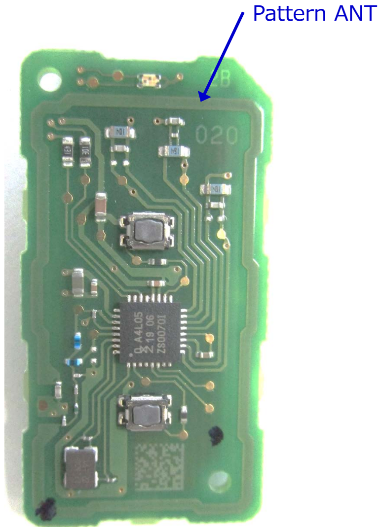
FRONT VIEW
