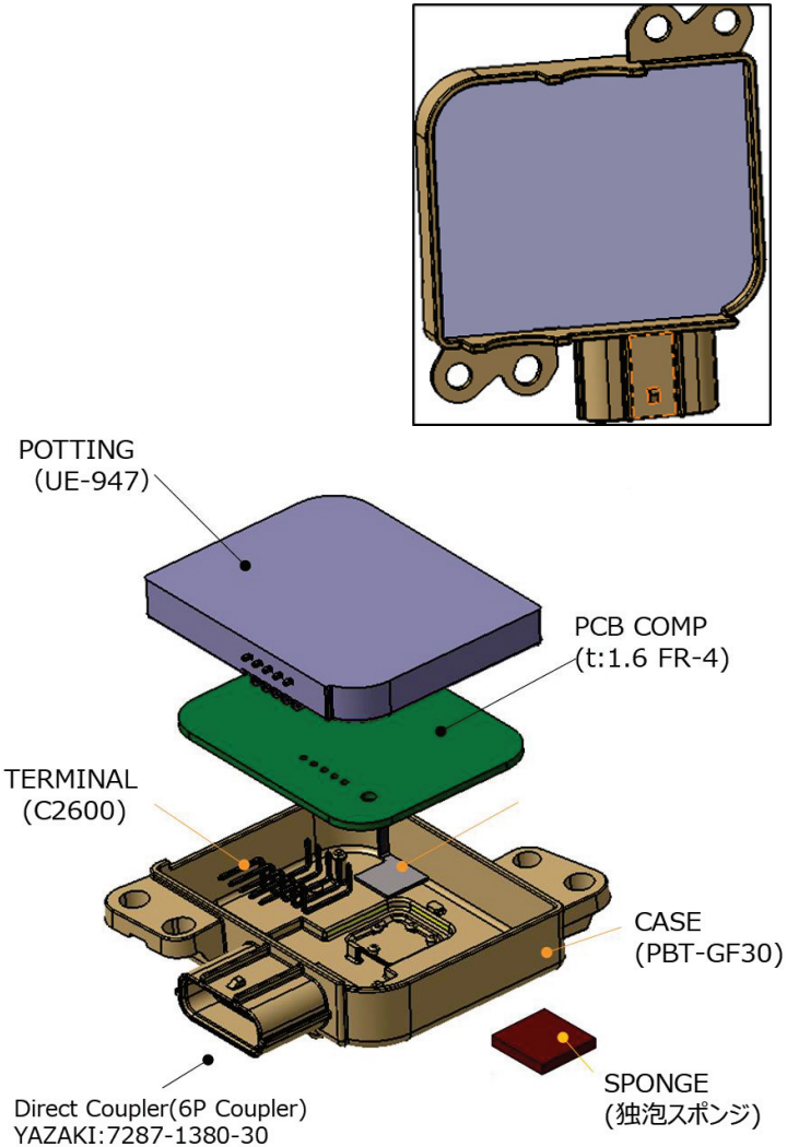
EXT NFC internal structure
