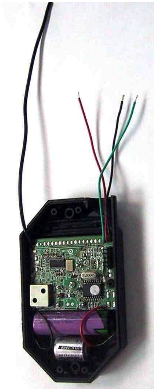
Photograph No.2 SpeedRead transmitter Internal view
