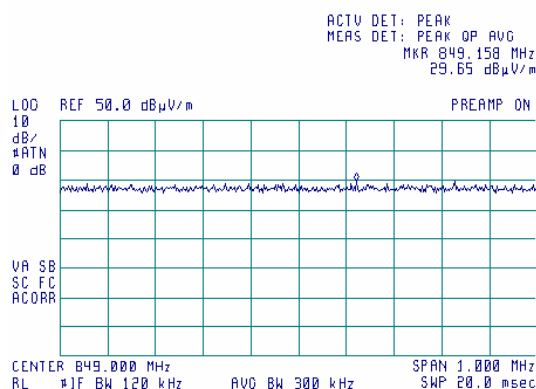
Plot 7.7.34 Radiated emission measurements at the 5 th harmonic
