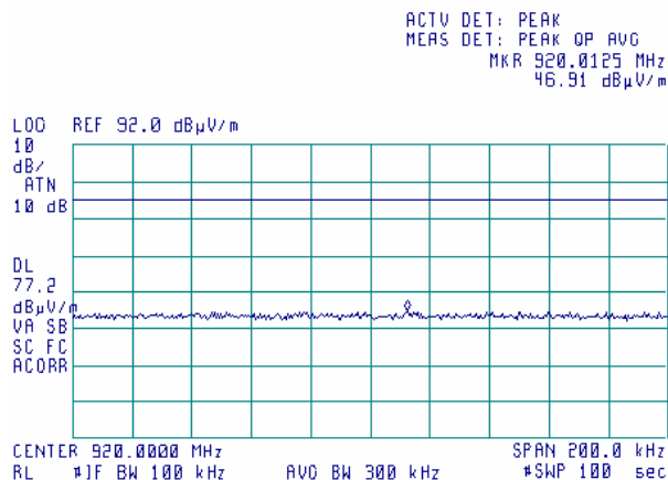
Plot 7.7.16 Radiated emission measurements at the 2 nd harmonic
