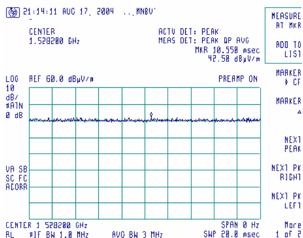
Plot 7.5.61 Radiated emission measurements at the 9 th harmonic
