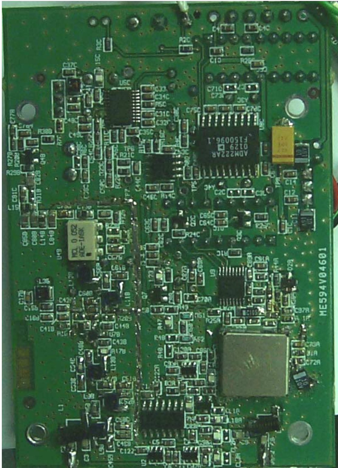
Photograph No.1 SPEED HPRx450 internal view main PCB
