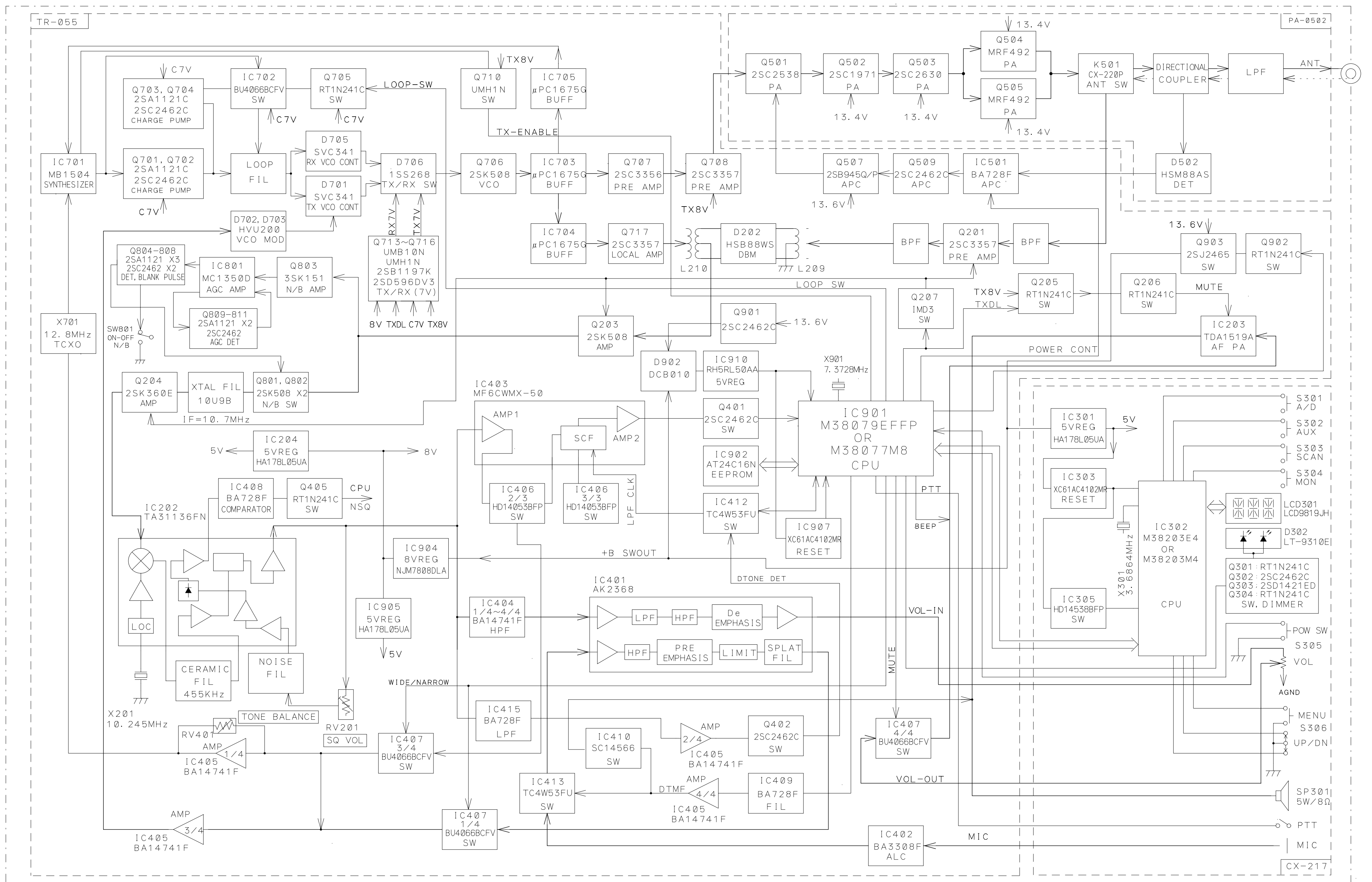
70-0671 BLOCK DIAGRAM
