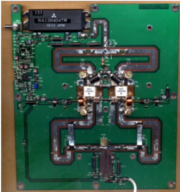
PA PCB Top View
