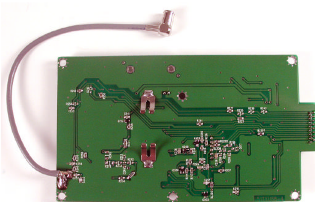
Transceiver PCB Bottom View
