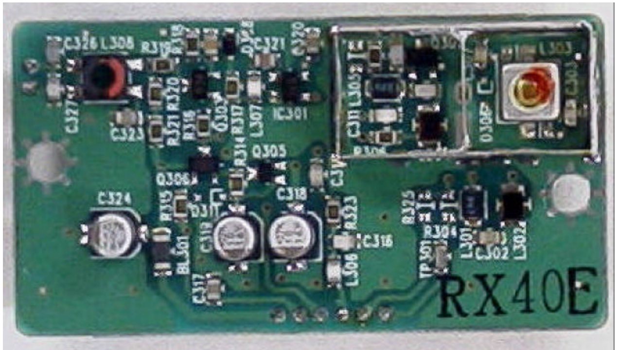
Receiver VC PCB Top View
