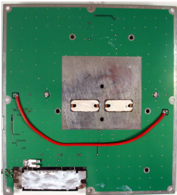
PA PCB Bottom View
