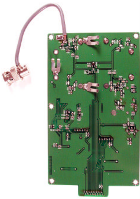
Receiver PCB Bottom View
