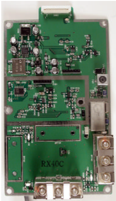
Receiver PCB Top View
