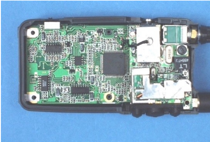
Mother & Daughter Boards w/Shields
