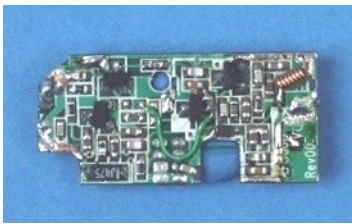
Daughter Board A W/O Shield
