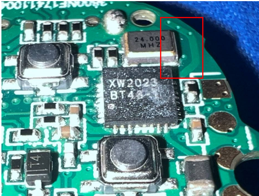
BT Antenna - back
