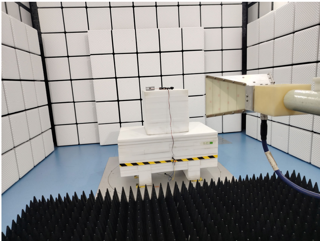
Radiated Spurious Emission - Back View (Above 1GHz)
