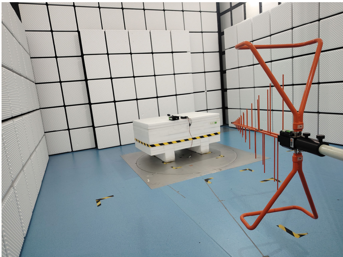
Radiated Spurious Emission - Back View (Below 1GHz)
