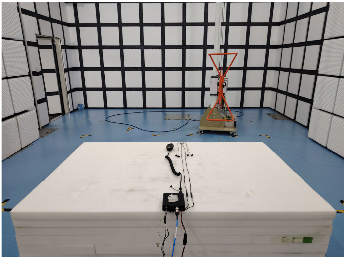
RE - Back View (Below 1GHz)
