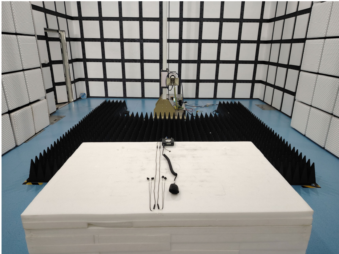
RE - Back View (Above 1GHz)
