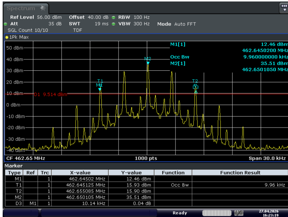
Test_Graph_GMRS_5W_462.65_12.5k_OBW
