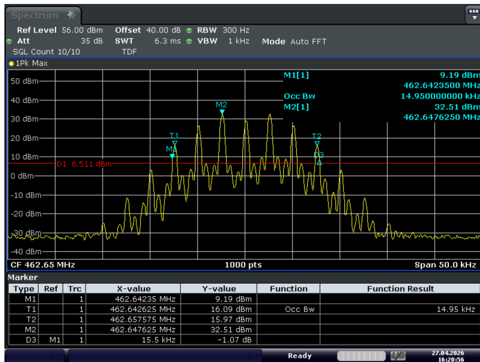
Test_Graph_GMRS_5W_462.65_12.5k_OBW
