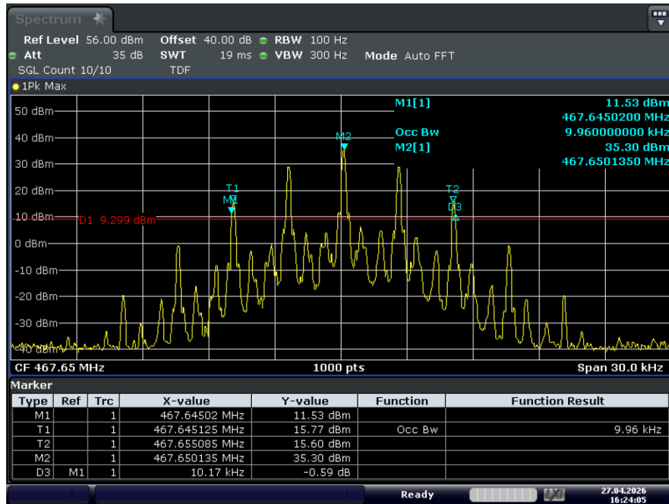
Test_Graph_GMRS_5W_467.65_12.5k_OBW
