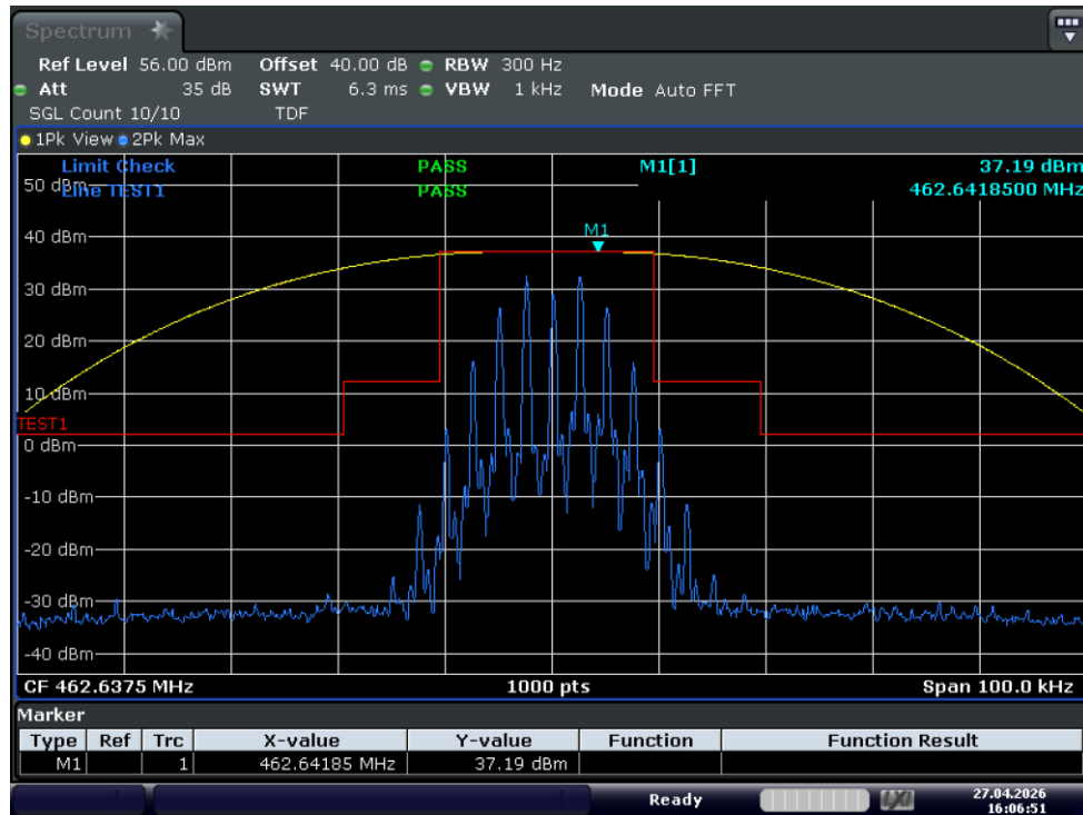
Test_Graph_GMRS_5W_462.6375_25k_Mask
