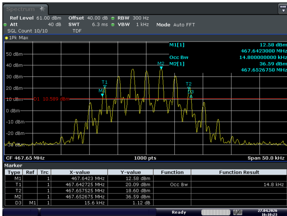
Test_Graph_GMRS_15W_467.65_12.5k_OBW
