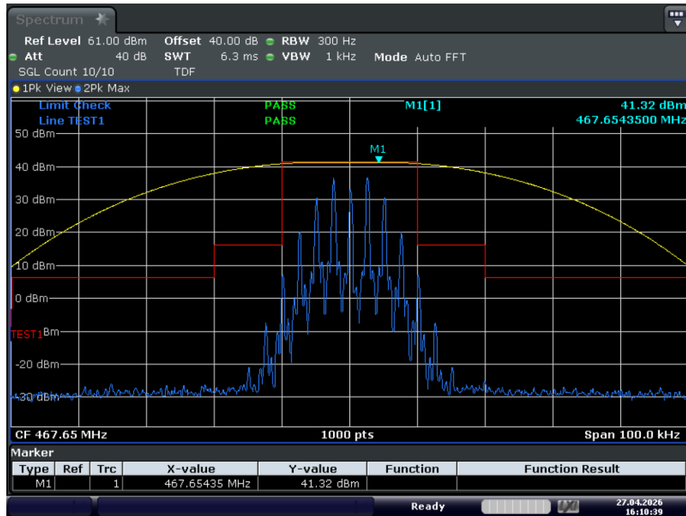
Test_Graph_GMRS_15W_467.65_25k_Mask
