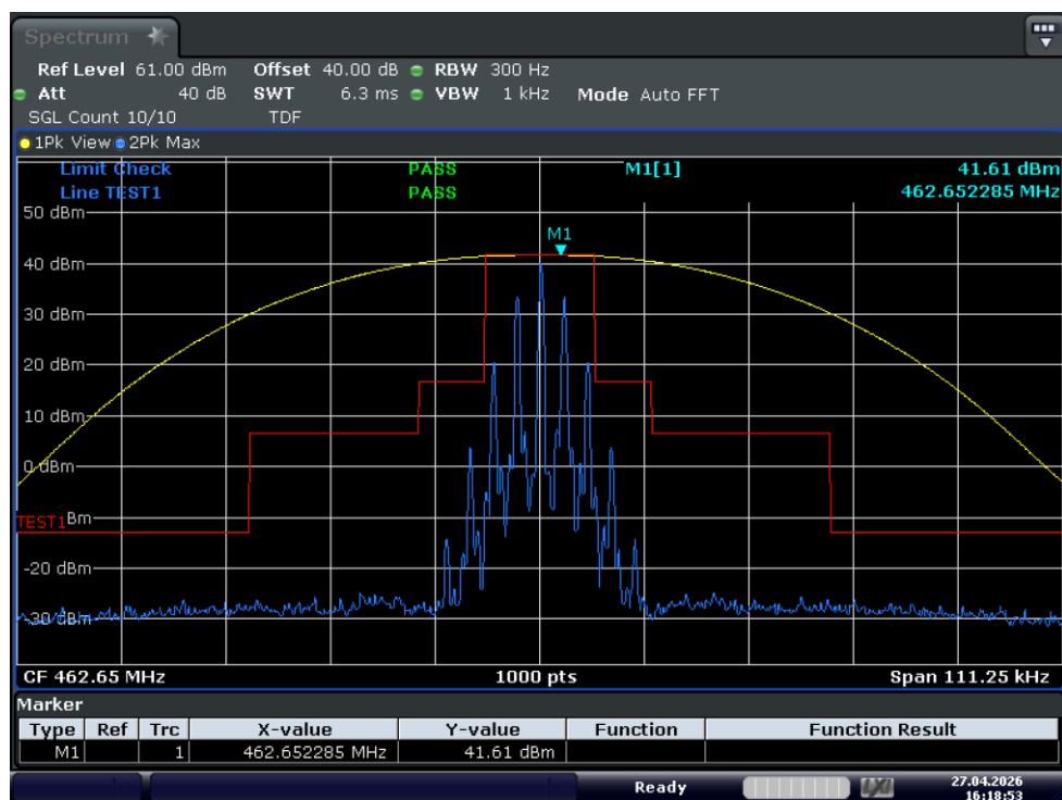
Test_Graph_GMRS_15W_462.65_12.5k_Mask
