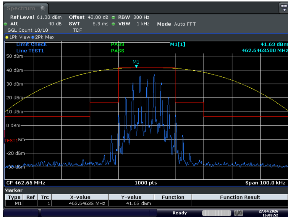
Test_Graph_GMRS_15W_462.65_25k_Mask
