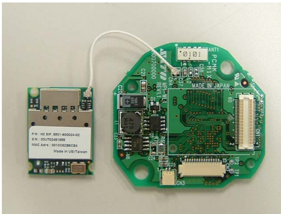
Wireless Module with Antenna and PWB
