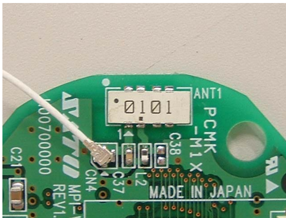
Antenna and PWB (zoomed) – Front
