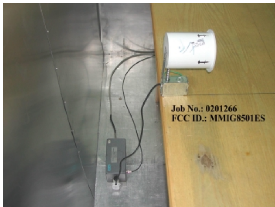
Side View
