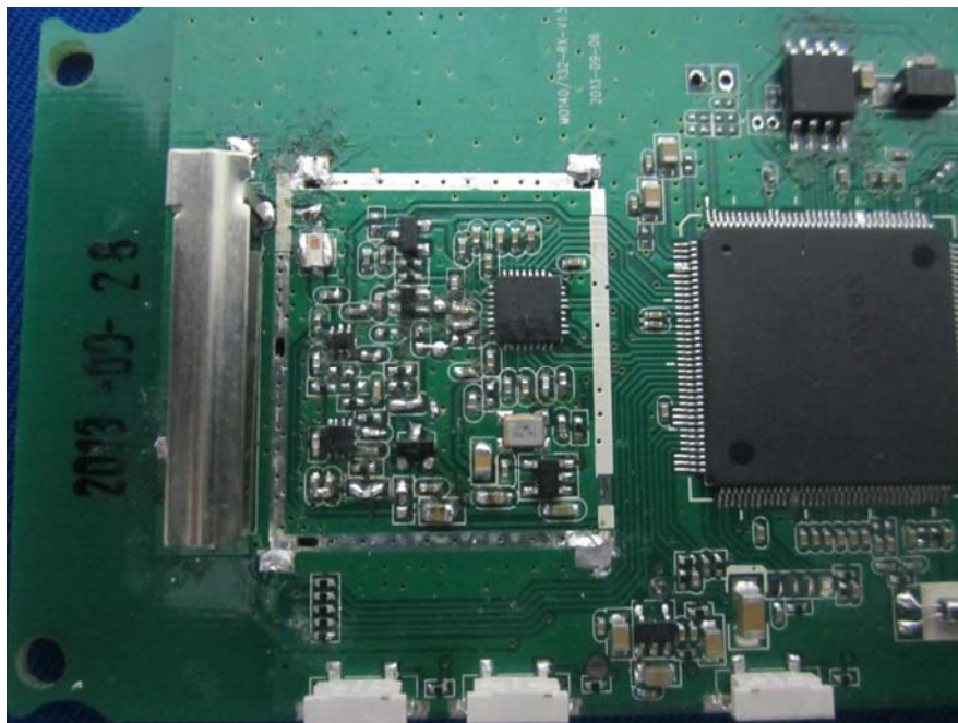
EUT –Shielding Case Uncover and Antenna View
