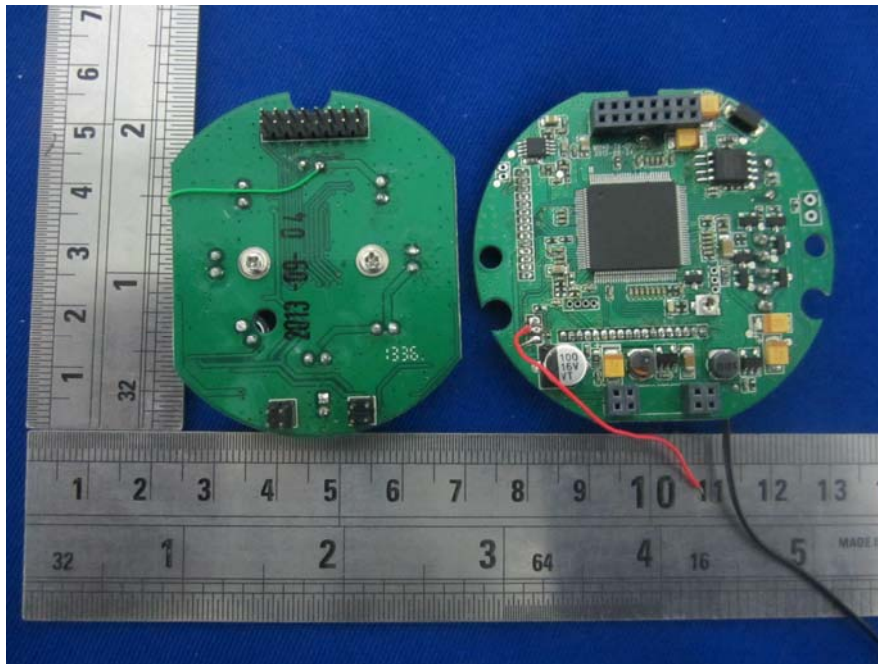
EUT – Camera Board Uncover View
