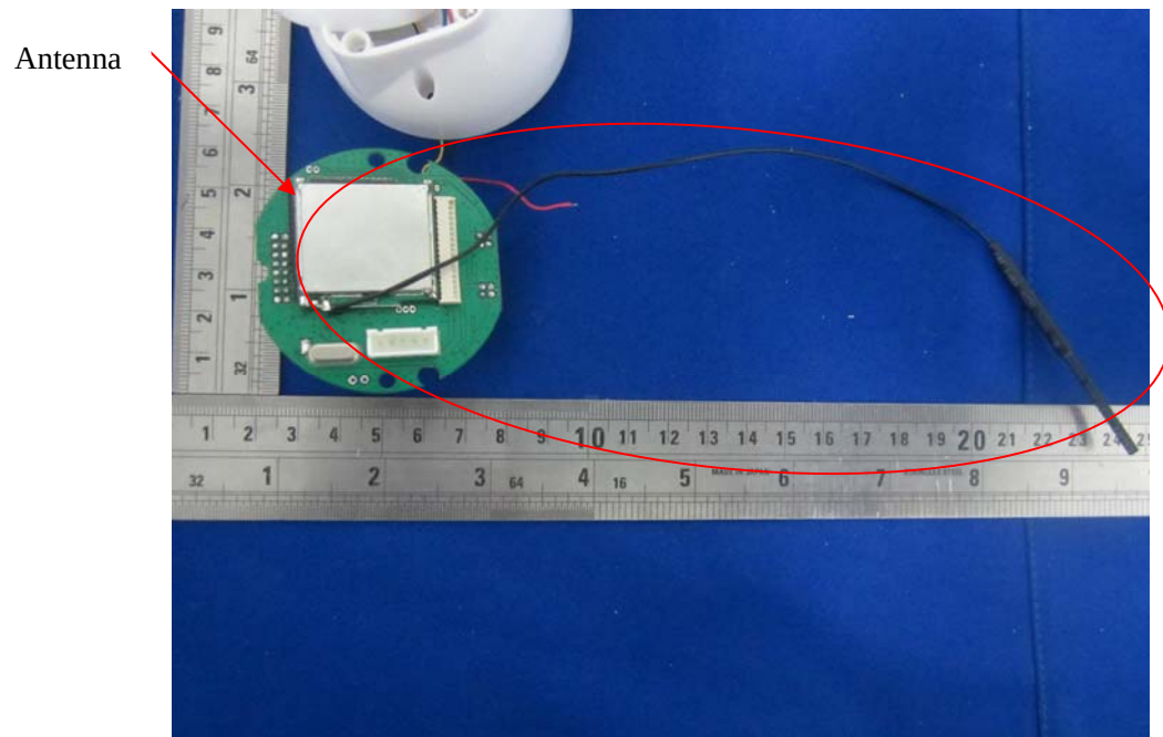
EUT – Camera Board Bottom With Shielding View
