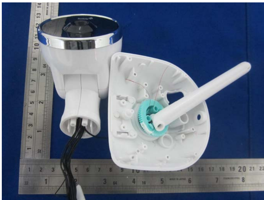
EUT – Control Uncover View
