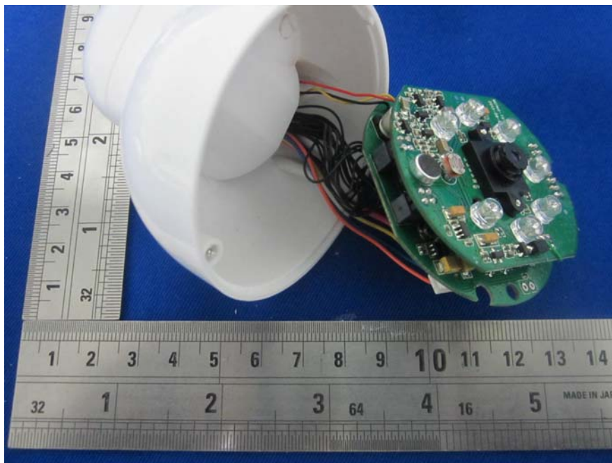
EUT – Camera Off View
