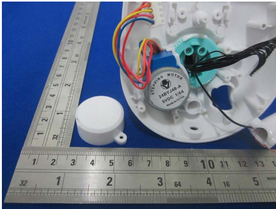
EUT – Motor Uncover View
