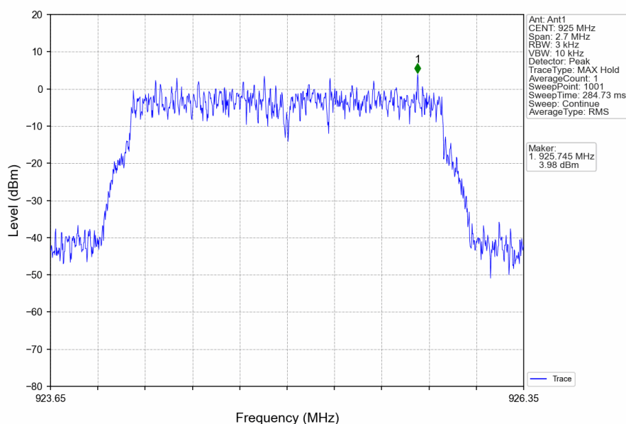
11ah_HCH_925MHz_Ant1_NTNV
