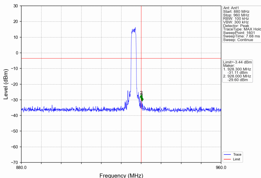
11ah_HCH_925MHz_Ant1_NTNV
