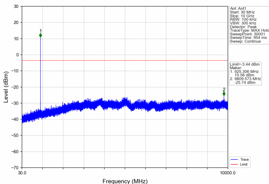
11ah_HCH_925MHz_Ant1_NTNV
