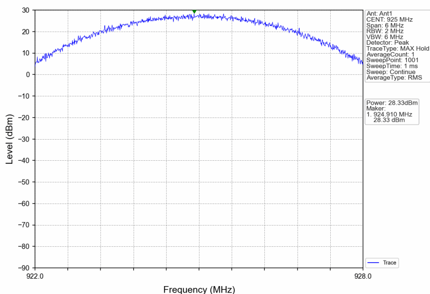
11ah_HCH_925MHz_Ant1_NTNV
