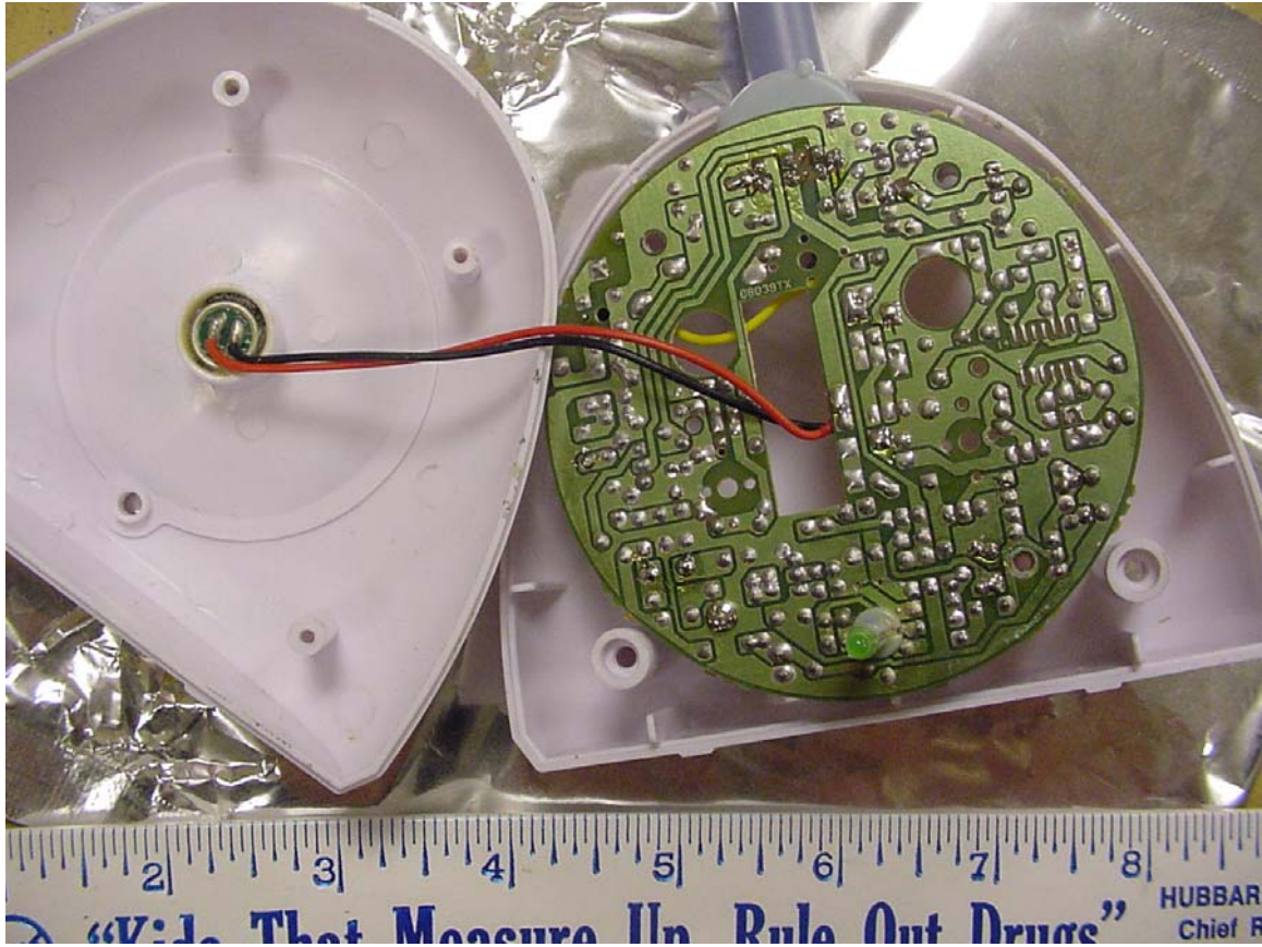
Interior with front cover removed showing solder side of PCB and microphone installation.
