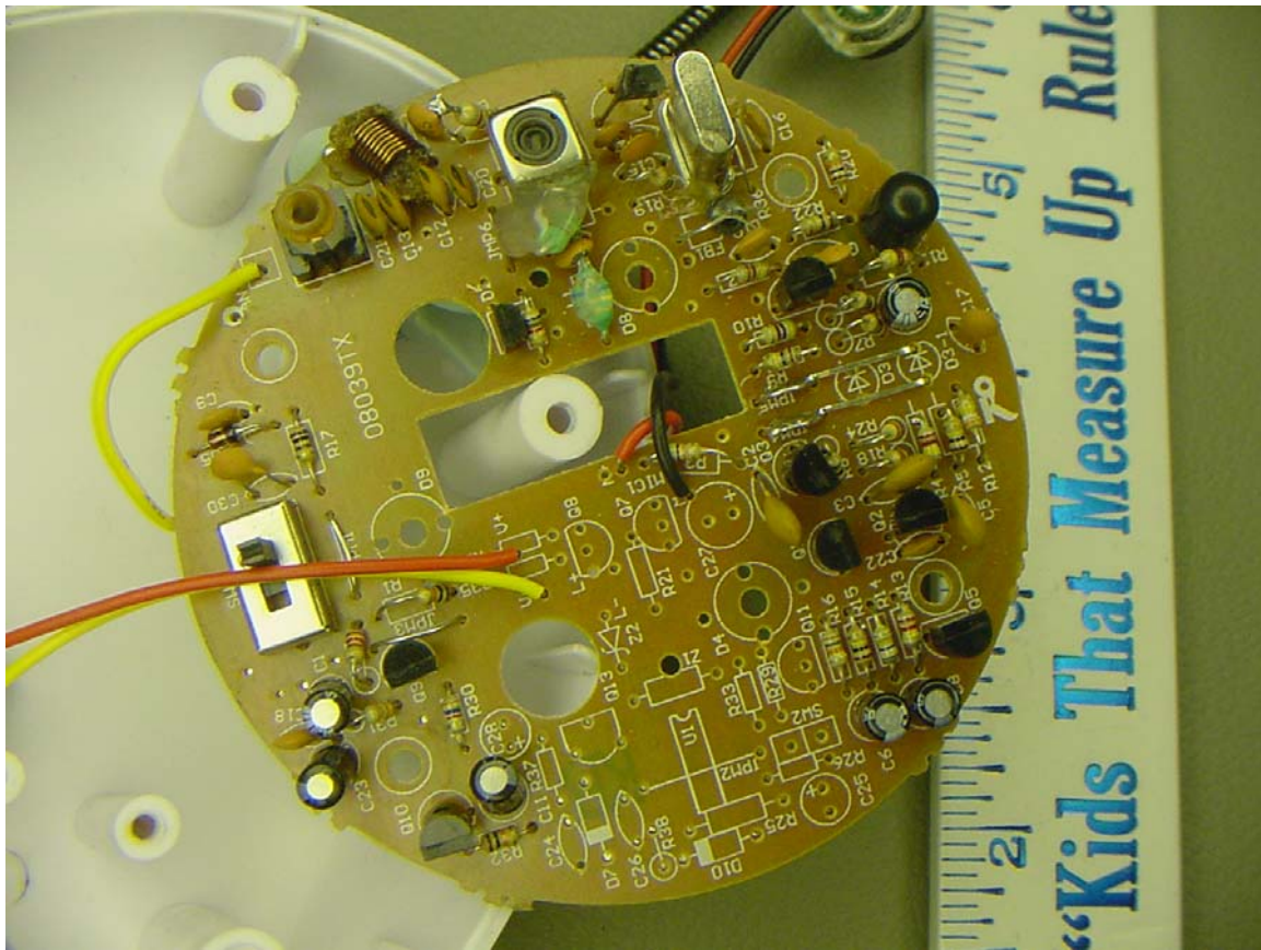
Component side of PCB
