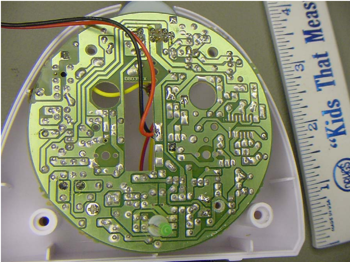
Solder side of PCB
