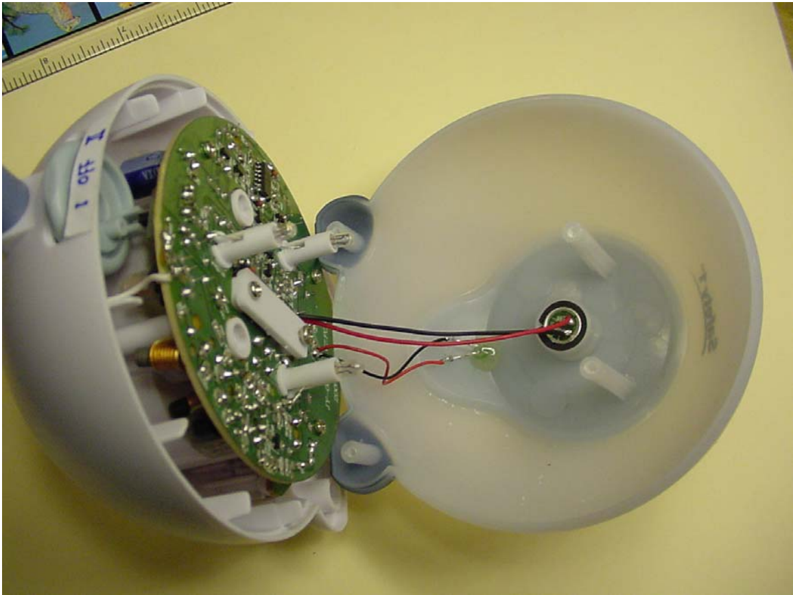
Inside view showing microphone and LED installation
