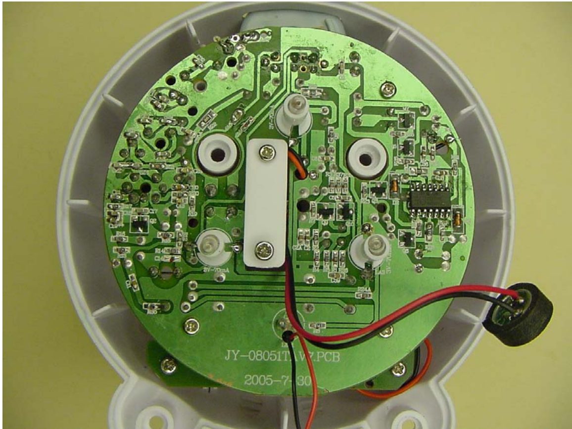
PCB Rear
