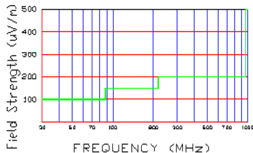
Figure 11. Spurious Radiated Limits at 3 meters
