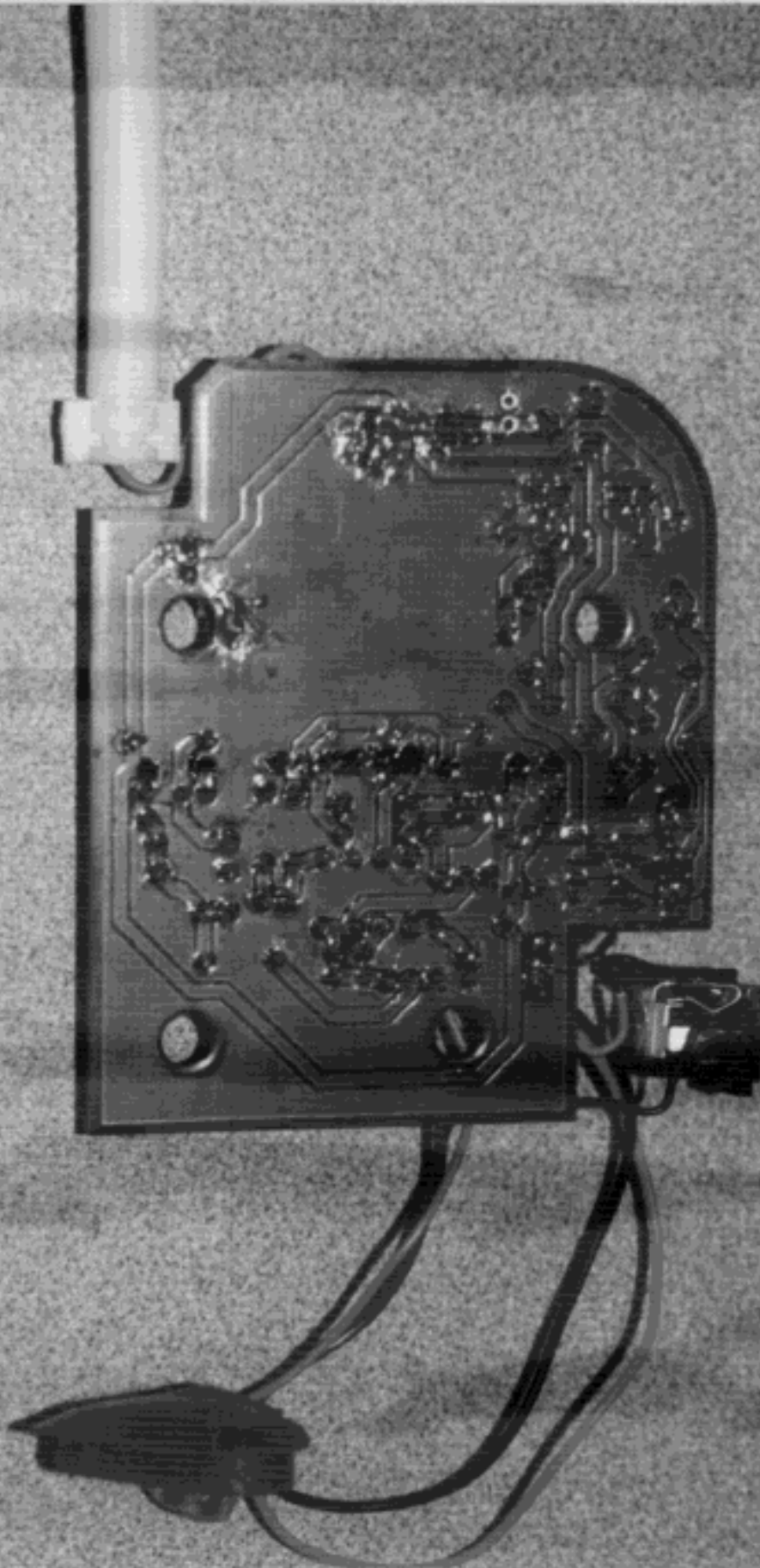
Figure 9.7 Controller PCB (Foil Side)
