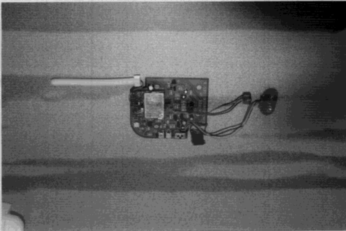
Figure 9.5 RF & Controller PCB Assembled
