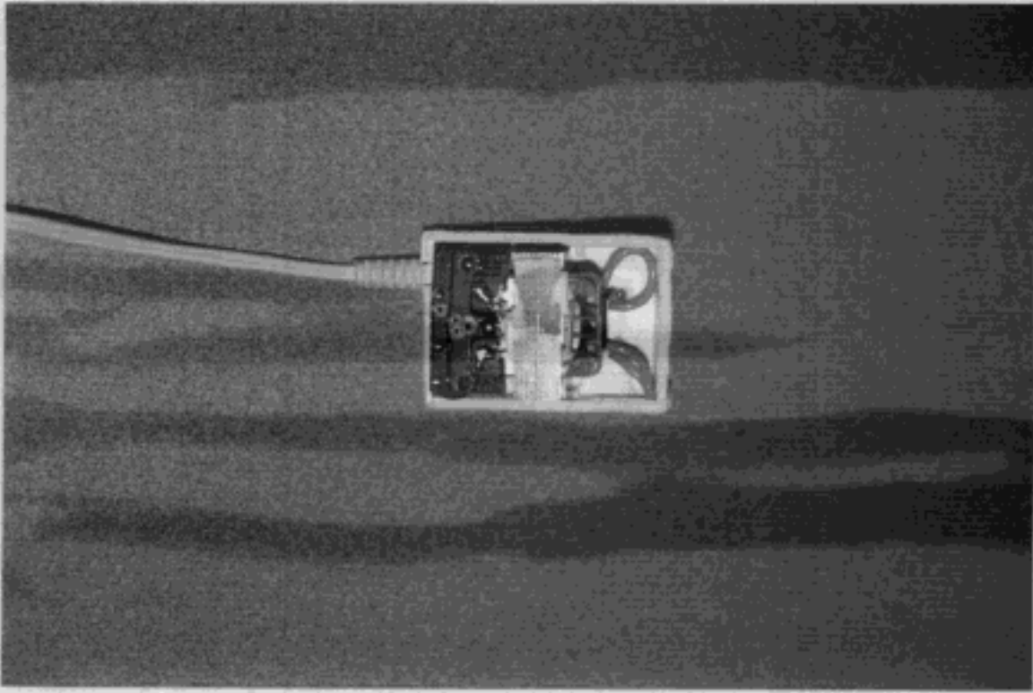
Figure 9.9 Bottom of Power Supply Board
