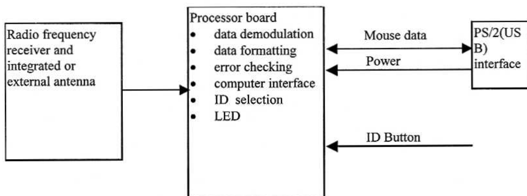
Figure 3. Receiver Block Diagram
