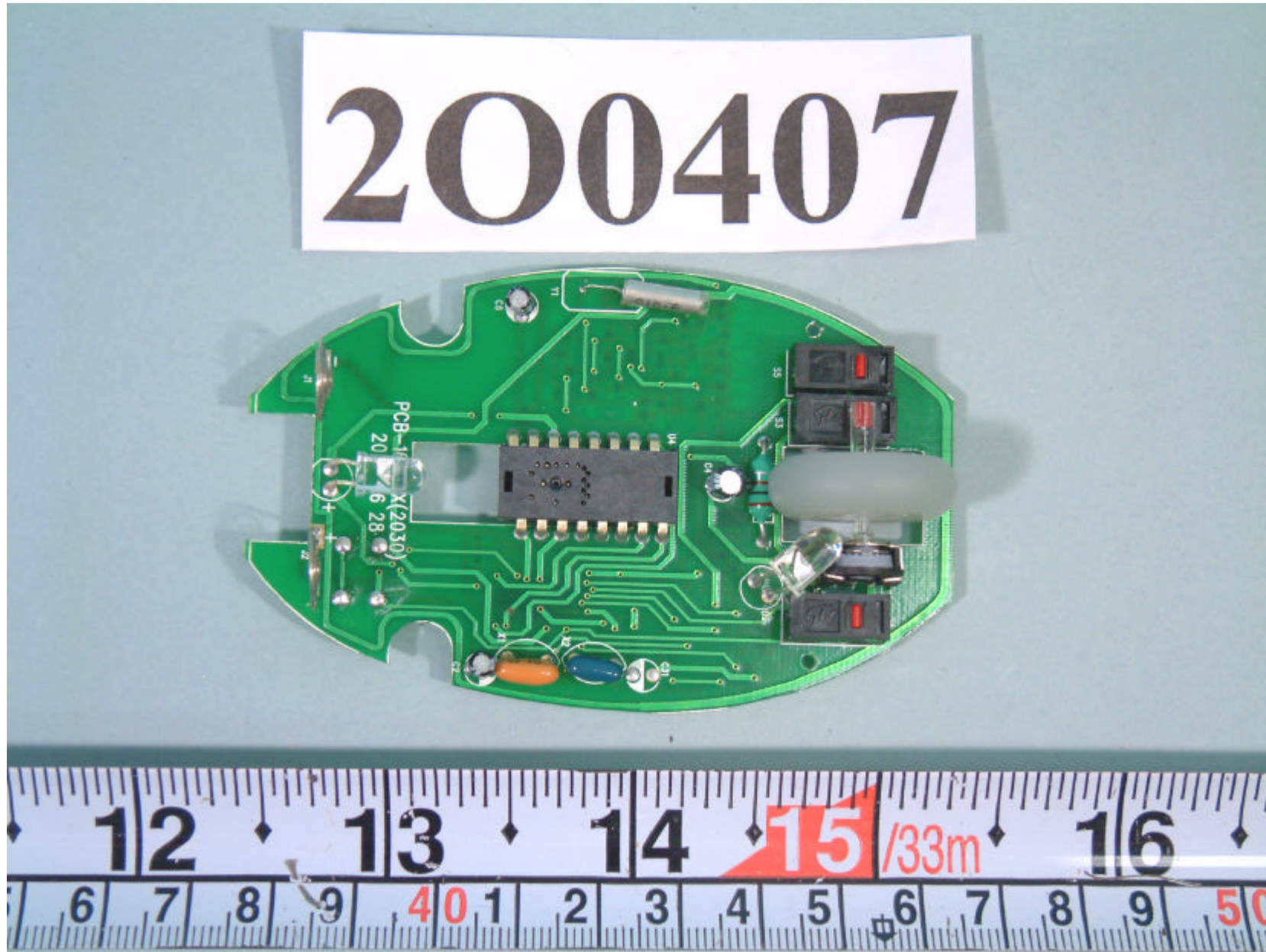
Front side of Main Board(MOUSE)
