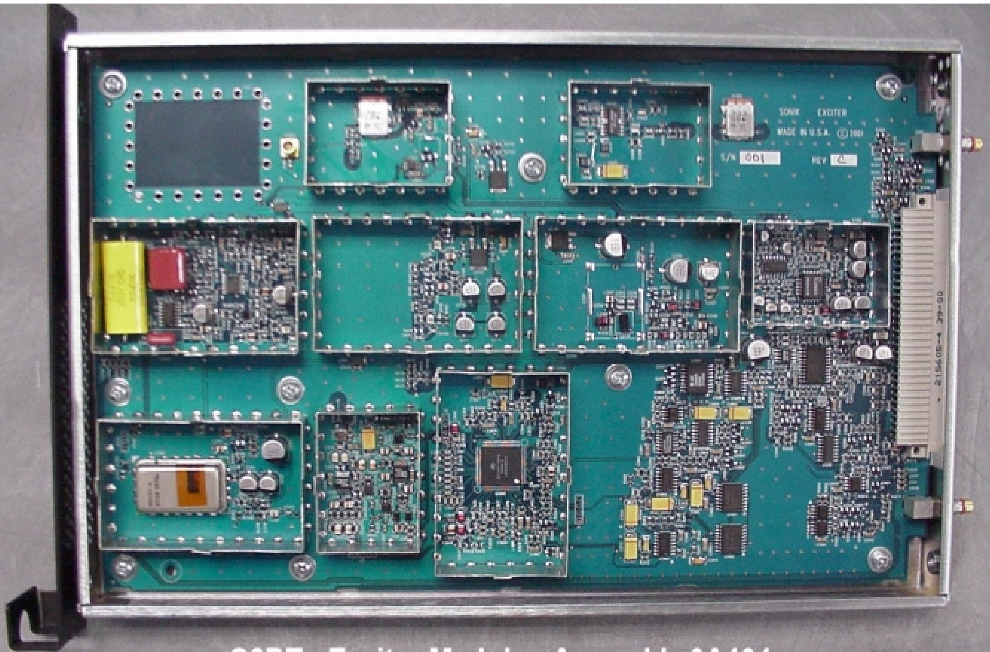
G2BT - Exciter Module - Assembly 6A401
