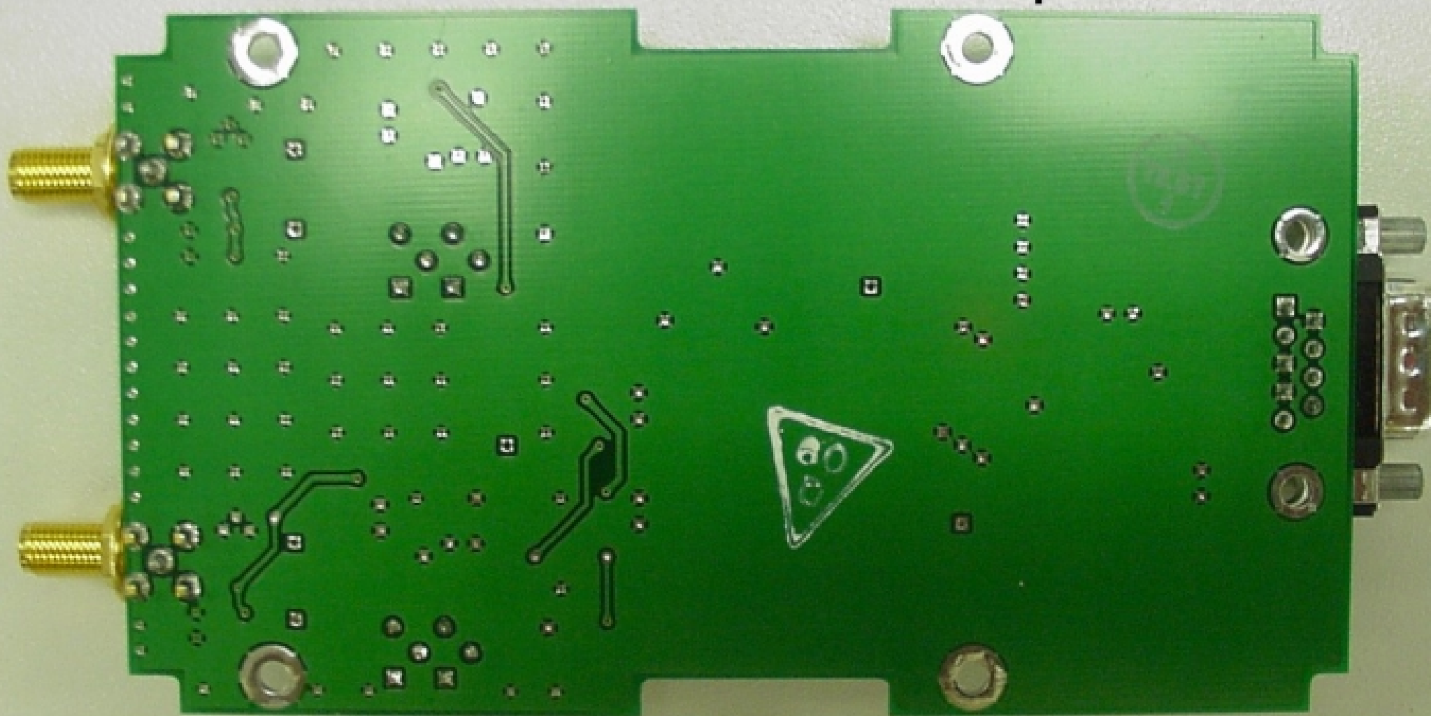
G2BT Power Detector PCB - Non Component View
