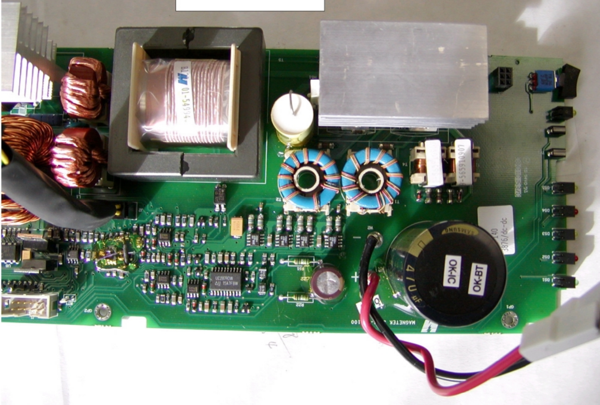
Power Supply part1.1 (top view)
