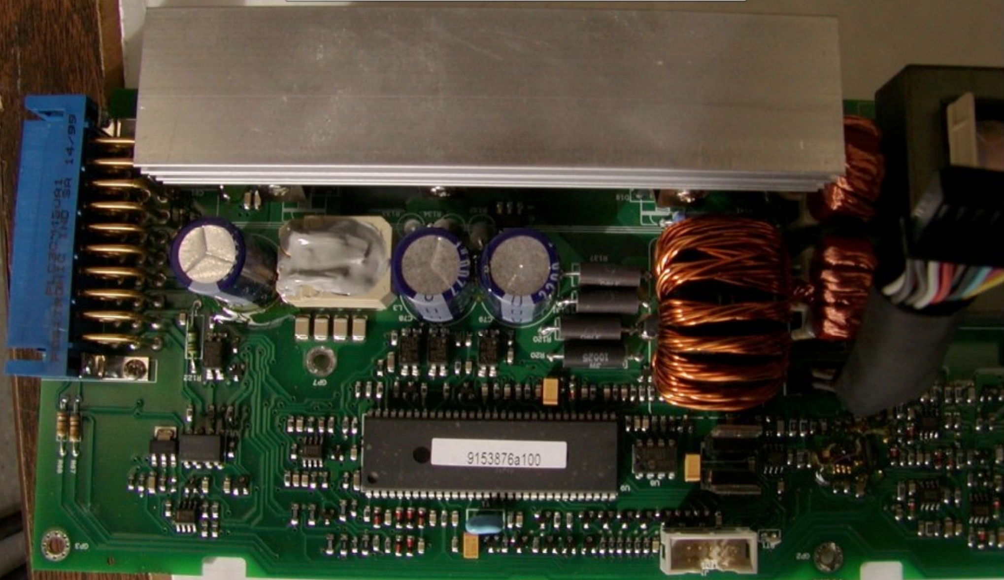
Power Supply part 1. 2 (top view)
