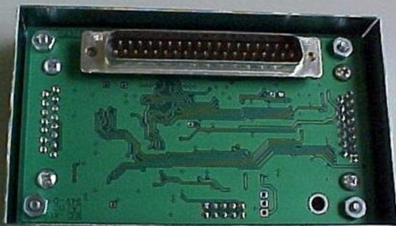
G2BT Power Supply SPI Interface Card (Cage Connector Side)
