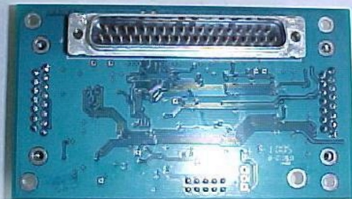
Power Supply SPI Interface Card
