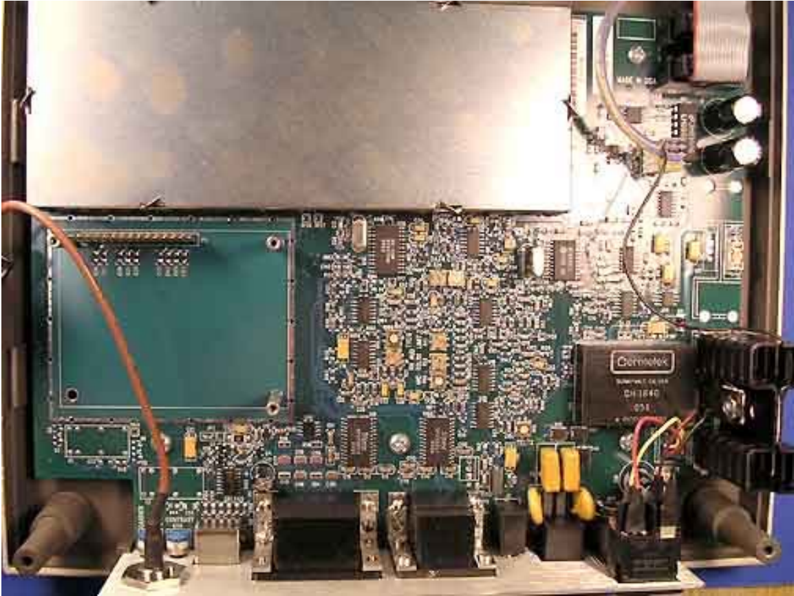
Controller PCB TX Module Removed
