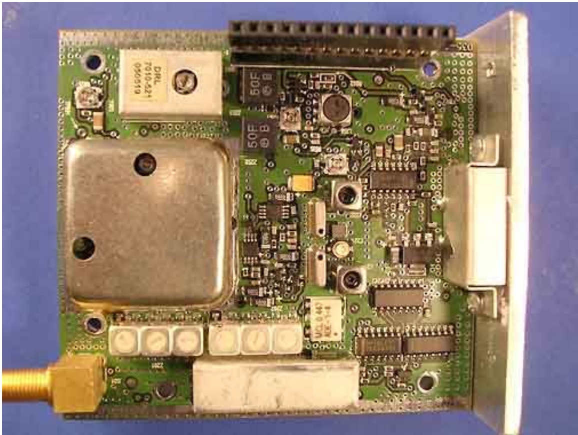
TX Module Exposed Top
