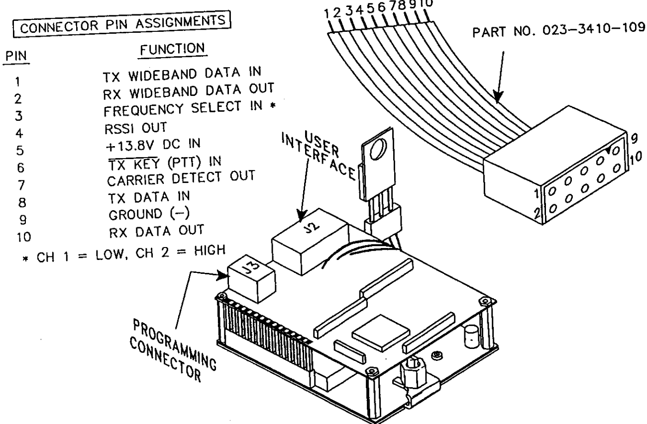
DL3472 WITH LOADER BOARD INTERFACE CABLE INSTALLATION FIGURE 2-2
