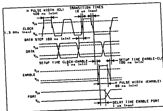
BUS TIMING FIGURE 3-2
