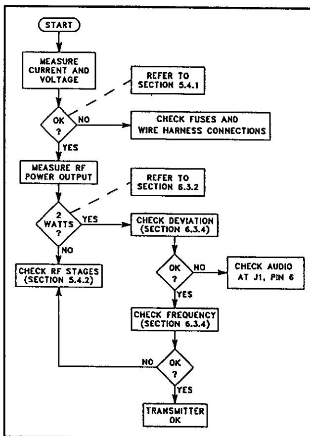
TRANSMITTER SERVICING FLOWCHART FIGURE 5-2
