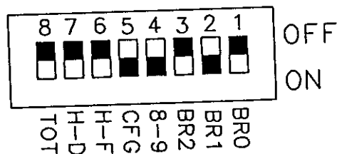
DIP SWITCH S2 FIGURE 2-5
