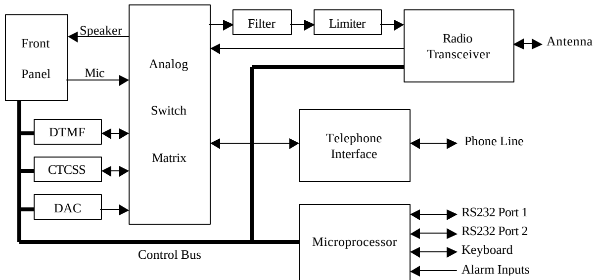
OSARC BASE Block Diagram
