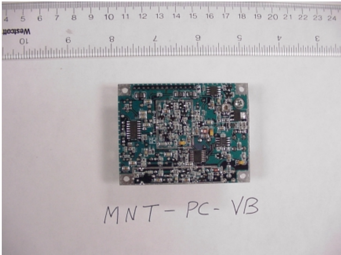
Bottom of RF board
