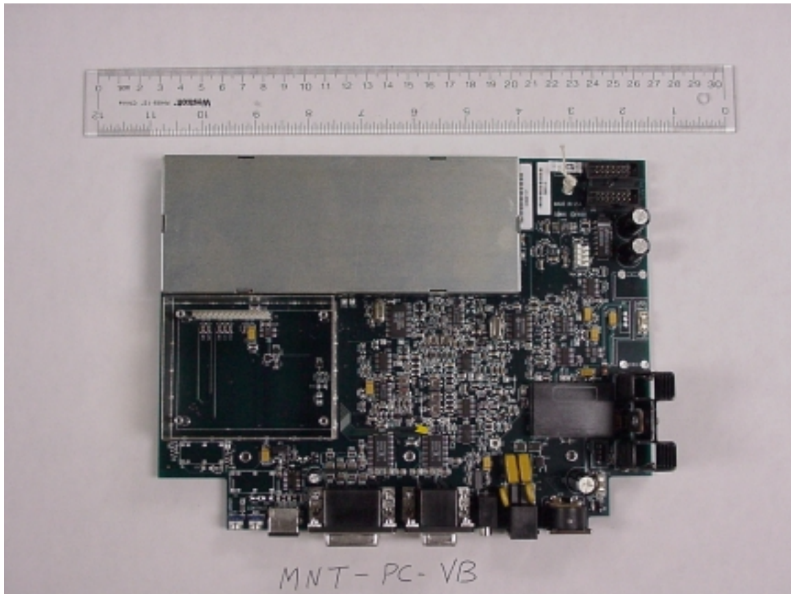
Top View of Main Board
