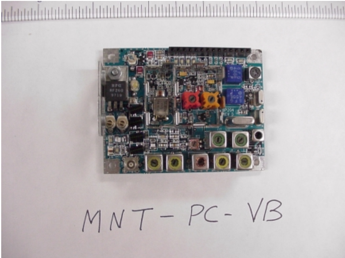
Top-side view of RF board
