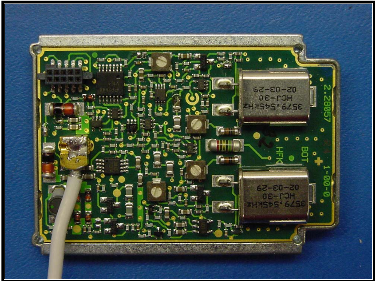
PHOTOGRAPH 47: MODULE RF PCB WITH OUT PORT TOP VIEW
