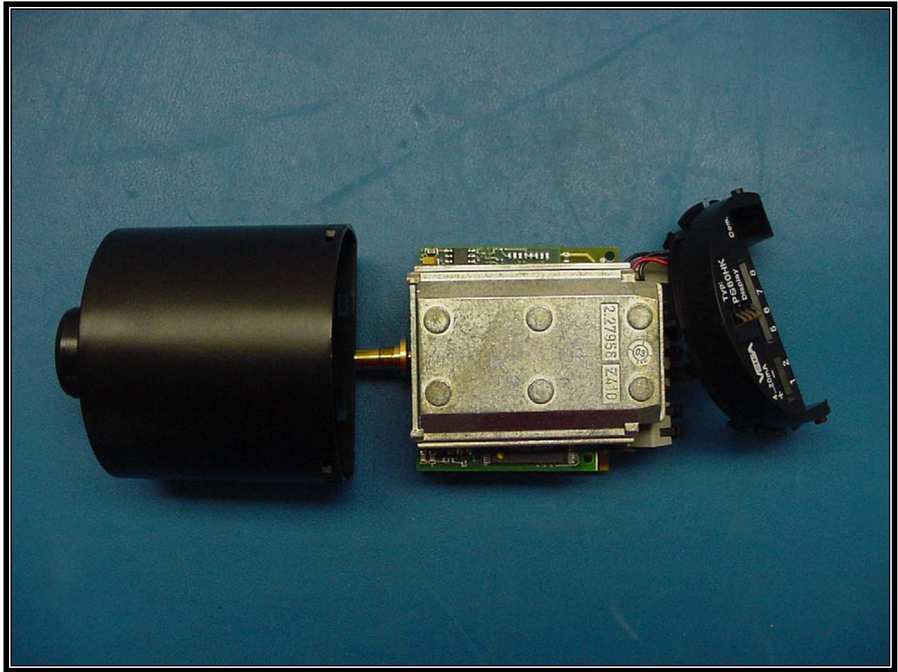
PHOTOGRAPH 39: EUT MODULE PARTS INSIDE VIEW
