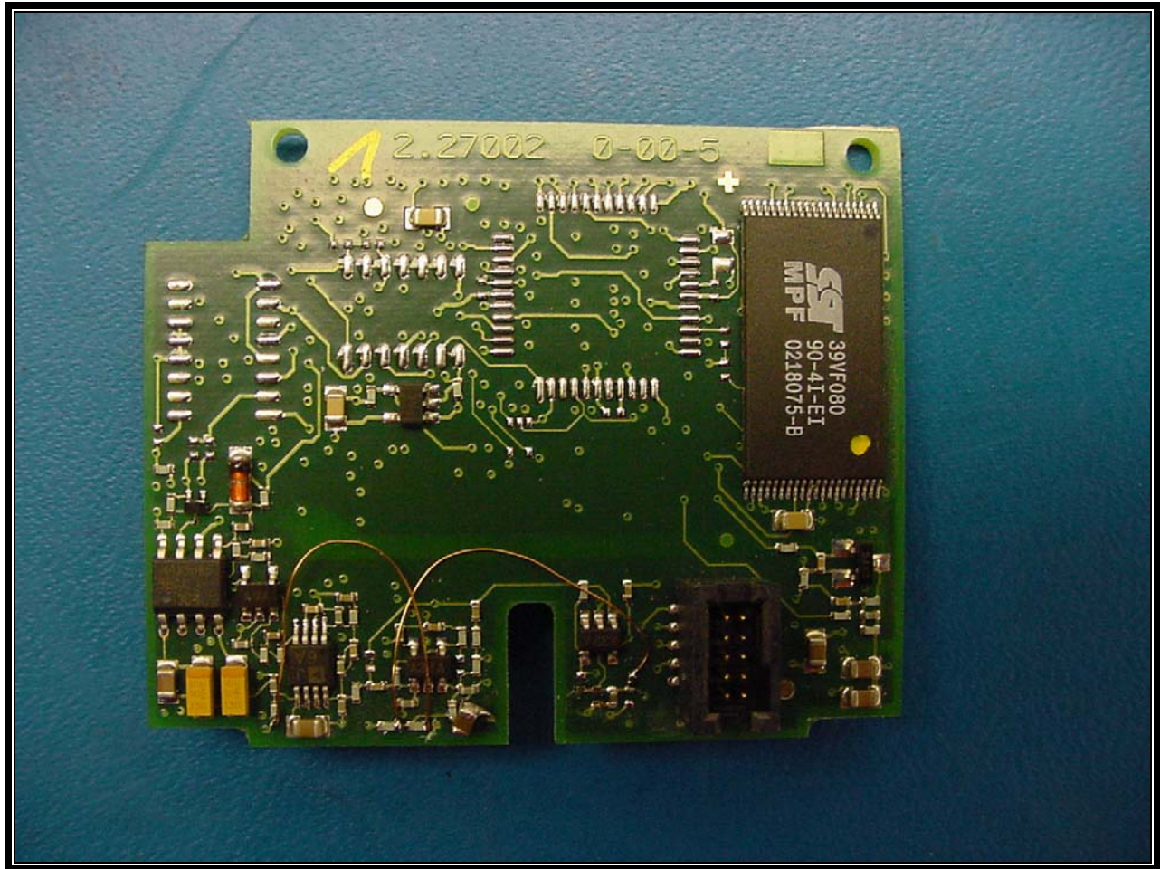
PHOTOGRAPH 44: MODULE PARTS PCB2 BOTTOM VIEW
