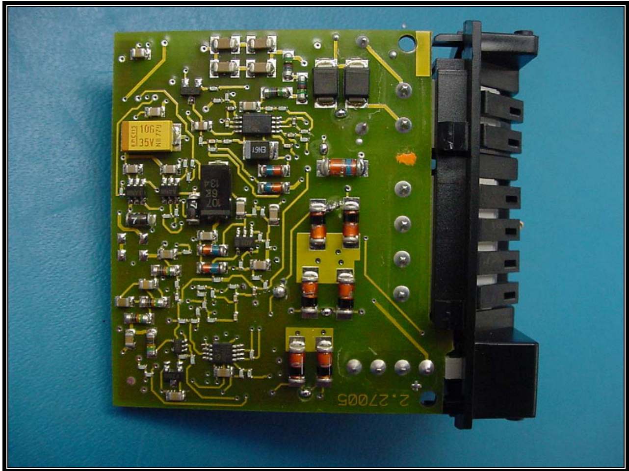
PHOTOGRAPH 42: EUT MODULE PARTS PCB1 BOTTOM VIEW
