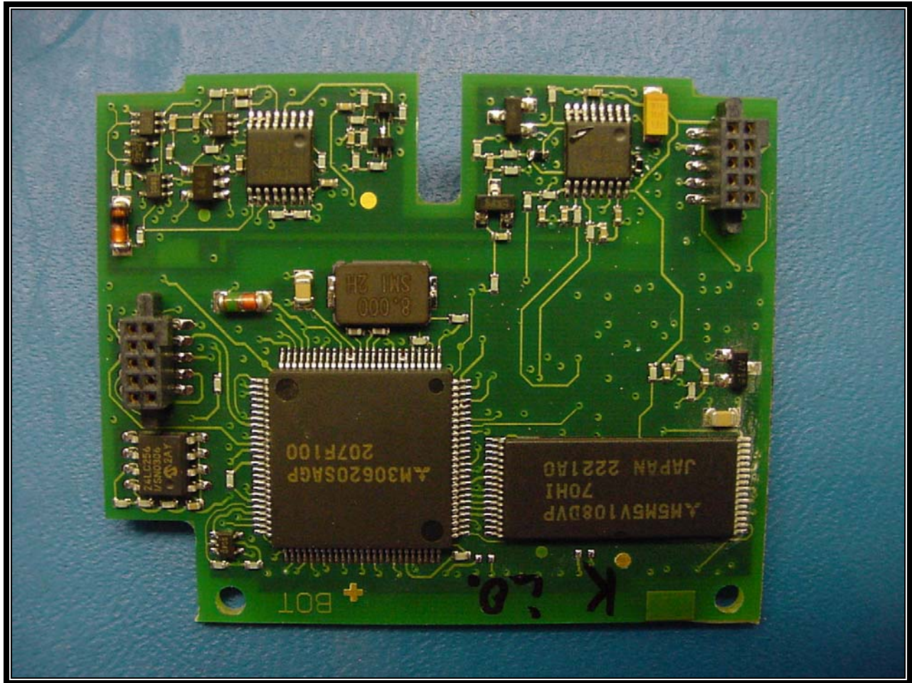
PHOTOGRAPH 45: MODULE PARTS PCB2 TOP VIEW
