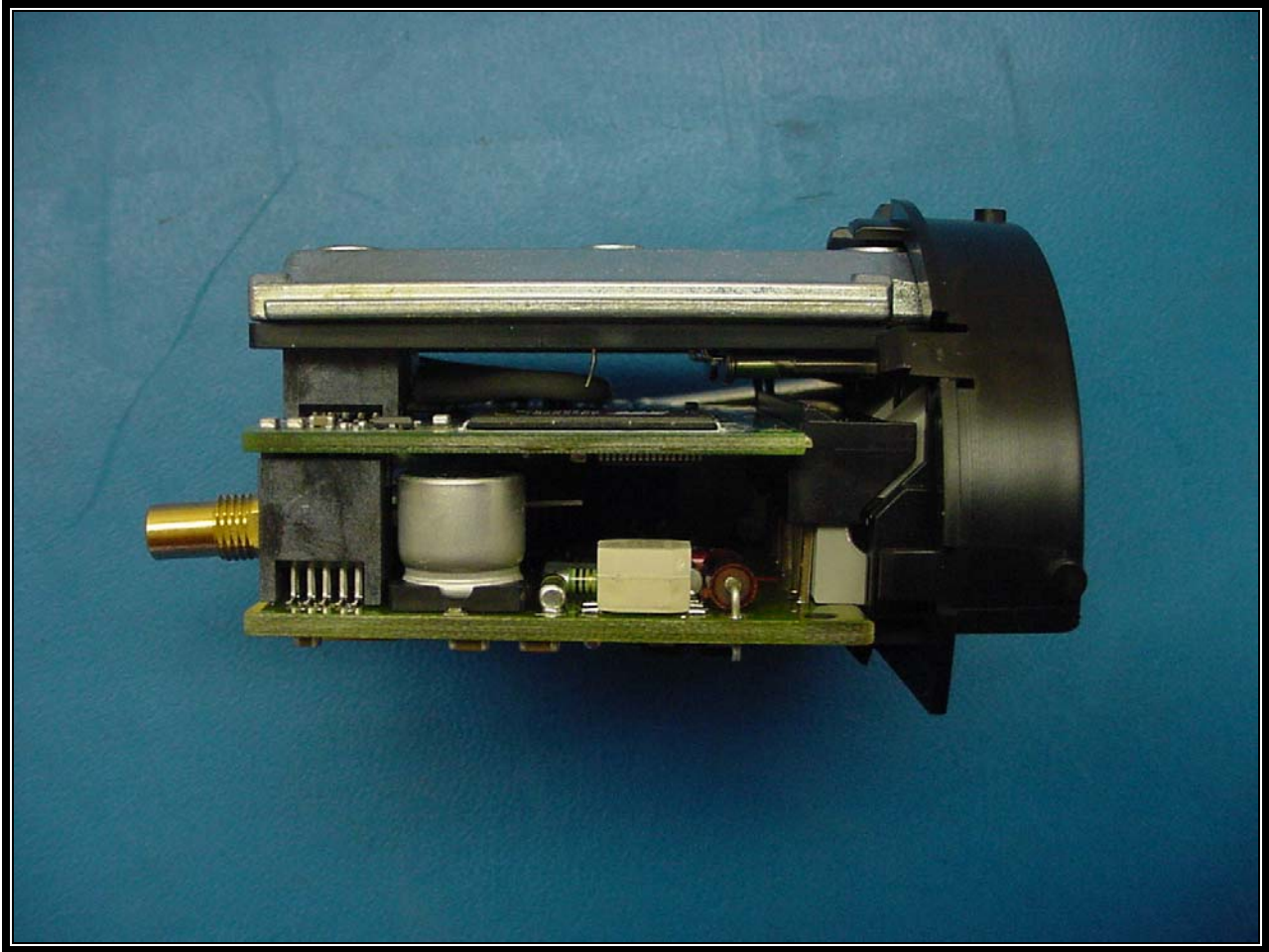
PHOTOGRAPH 40: EUT MODULE PARTS SIDE VIEW
