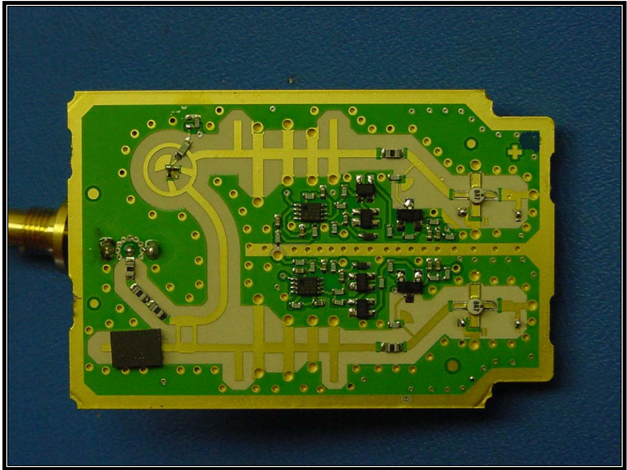
PHOTOGRAPH 48: MODULE RF PCB WITH OUT PORT BOTOM VIEW
