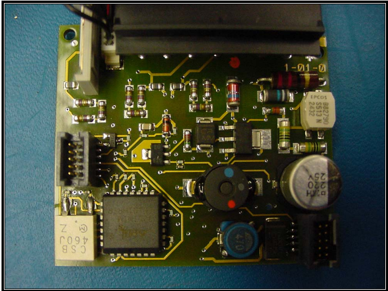
PHOTOGRAPH 43: MODULE PARTS PCB1 TOP VIEW
