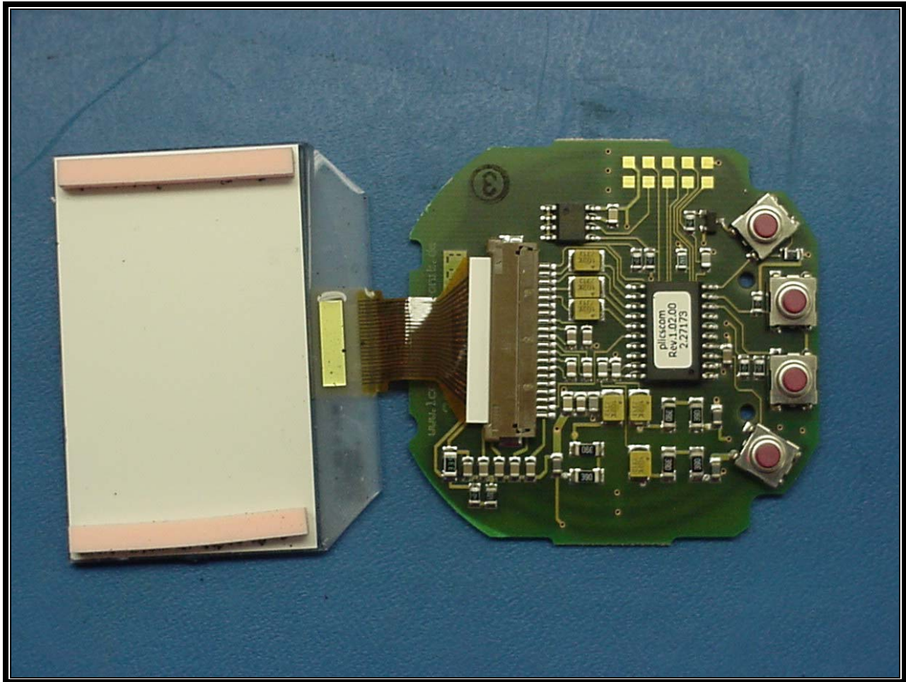
PHOTOGRAPH 34: EUT LCD DISPLAY-PCB BOTTOM VIEW
