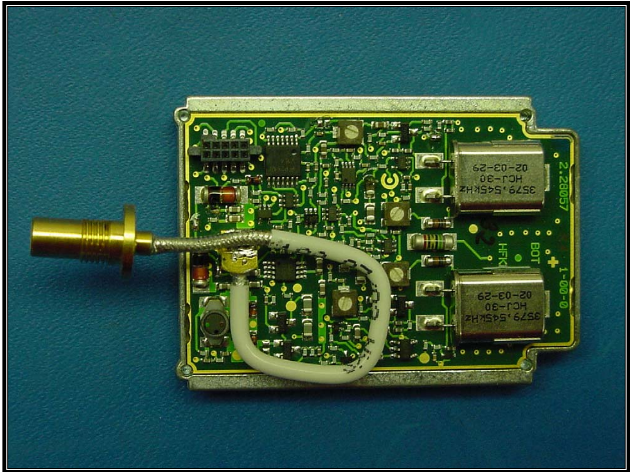
PHOTOGRAPH 46: MODULE RF PCB WITH PORT TOP VIEW
