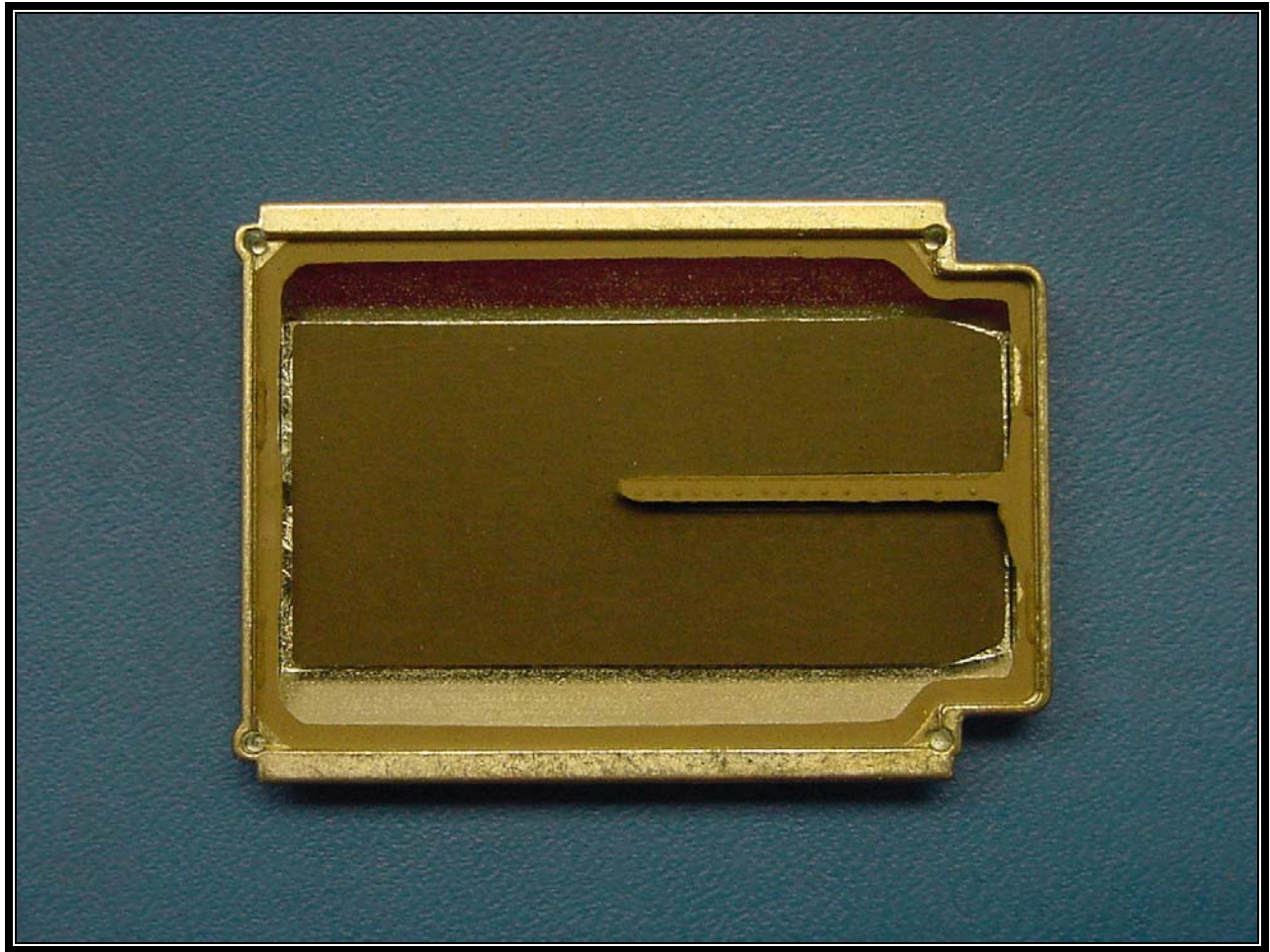
PHOTOGRAPH 49: MODULE RF PCB SHIELD TOP VIEW
