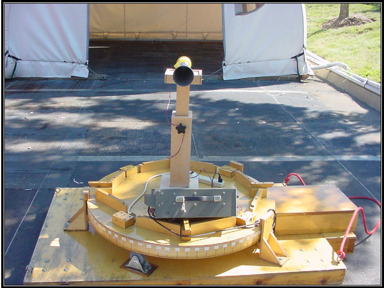
PHOTOGRAPH 6: RADIATED EMISSIONS FRONT VIEW 24.7DBI HORN
