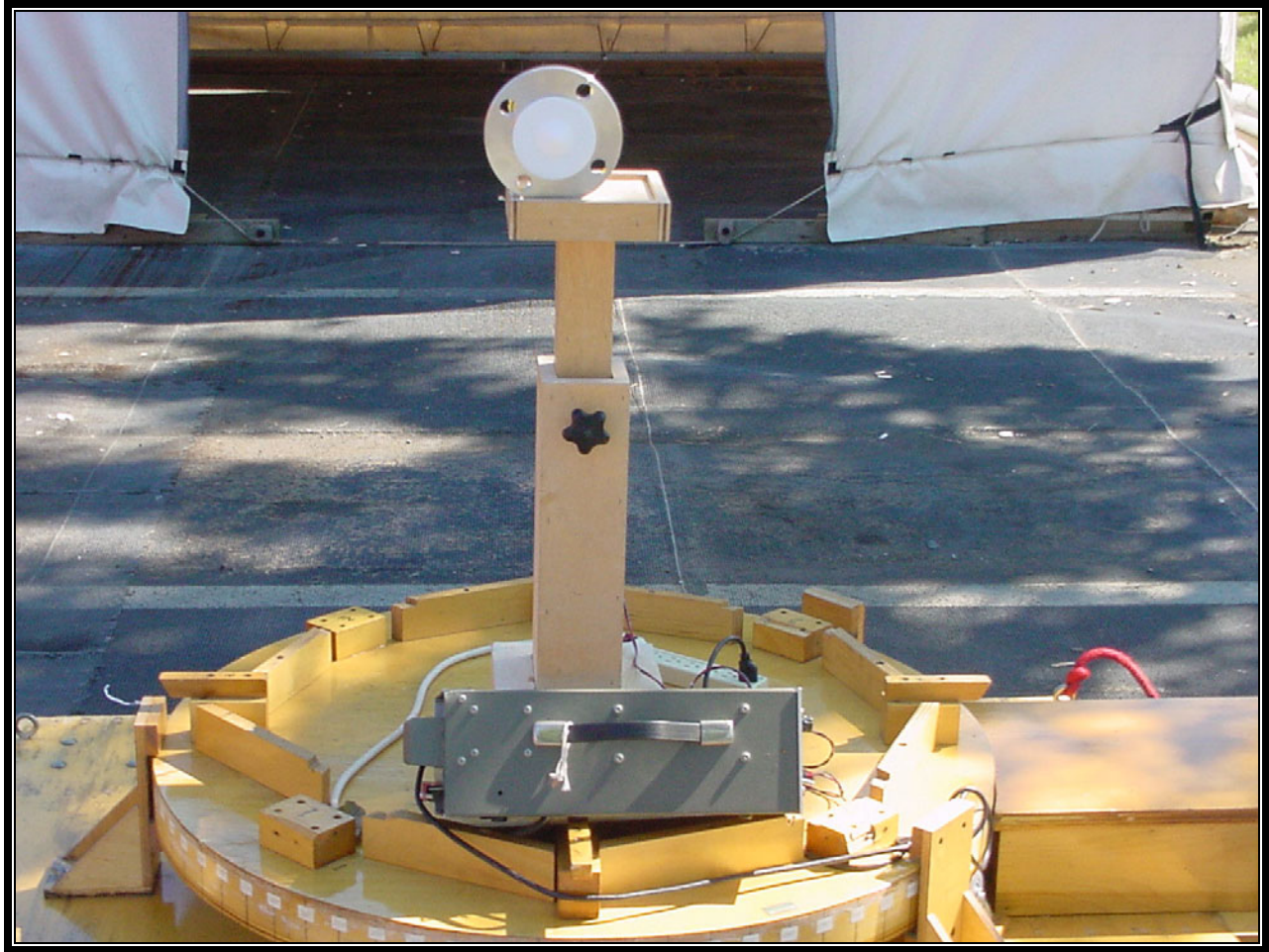
PHOTOGRAPH 9: RADIATED EMISSIONS REAR VIEW 21.2DBI HORN
