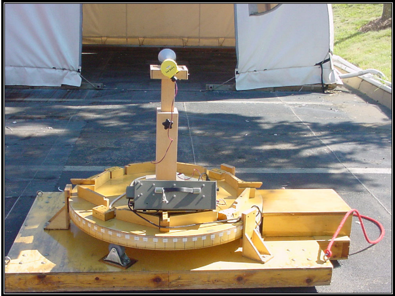
PHOTOGRAPH 7: RADIATED EMISSIONS FRONT VIEW 24.7DBI HORN
