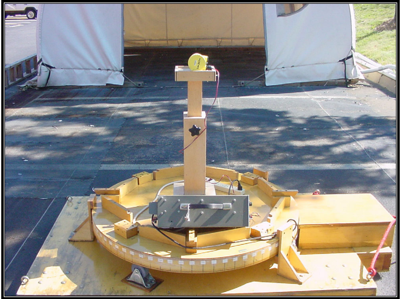
PHOTOGRAPH 5: RADIATED EMISSIONS REAR VIEW 19.5DBI ROD
