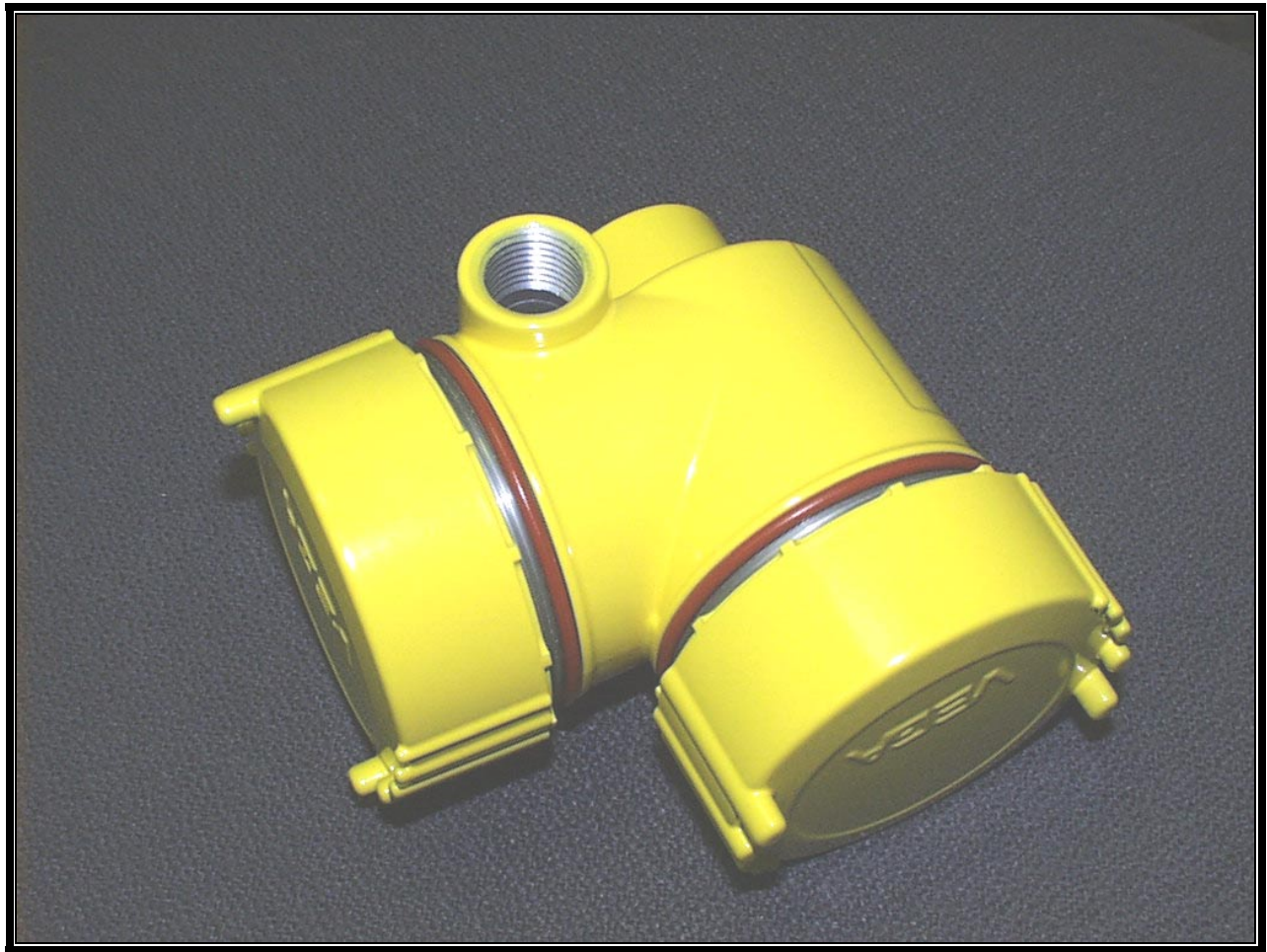
PHOTOGRAPH 9: EUT DOUBLE ALUMINUM CHAMBER HOUSING FITTING
