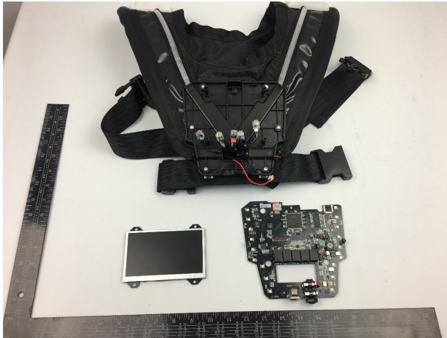
Front internal parts
