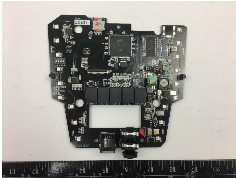
Front PCB – Top
