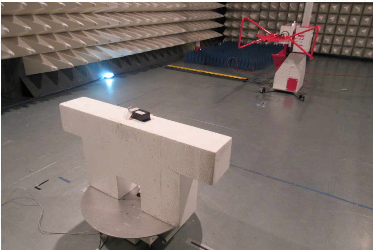
Radiated Emissions - above 1000 MHz
