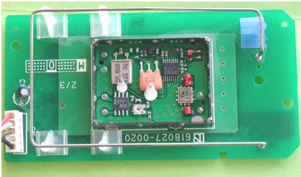
RE Receiver, Component Side
