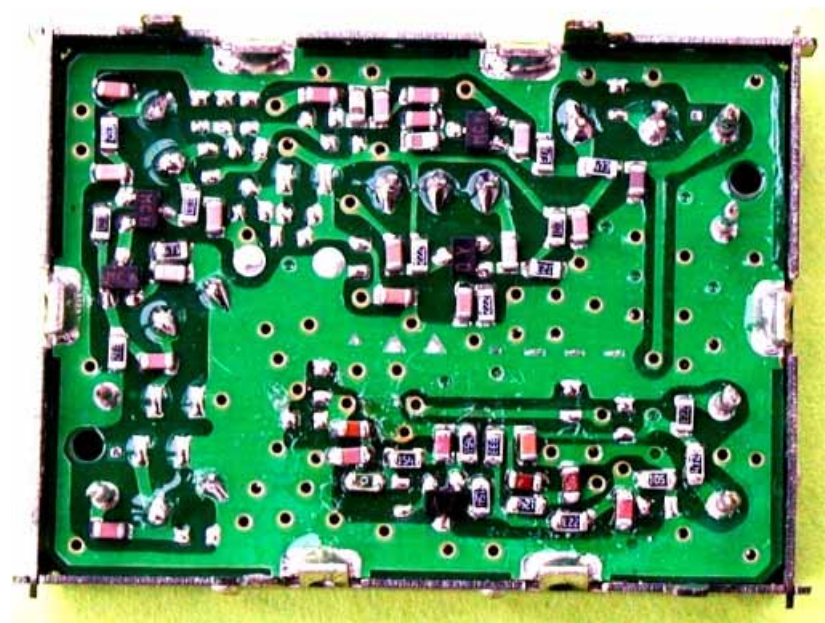
Receiver Module, Foil Side
