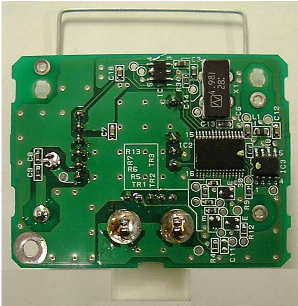
Receiver MDL B21RG Mother Board (Bottom view)
