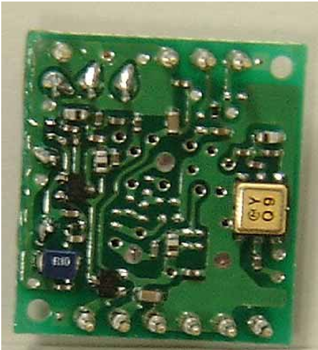
Receiver MDL B21RG RF Module (Bottom view)
