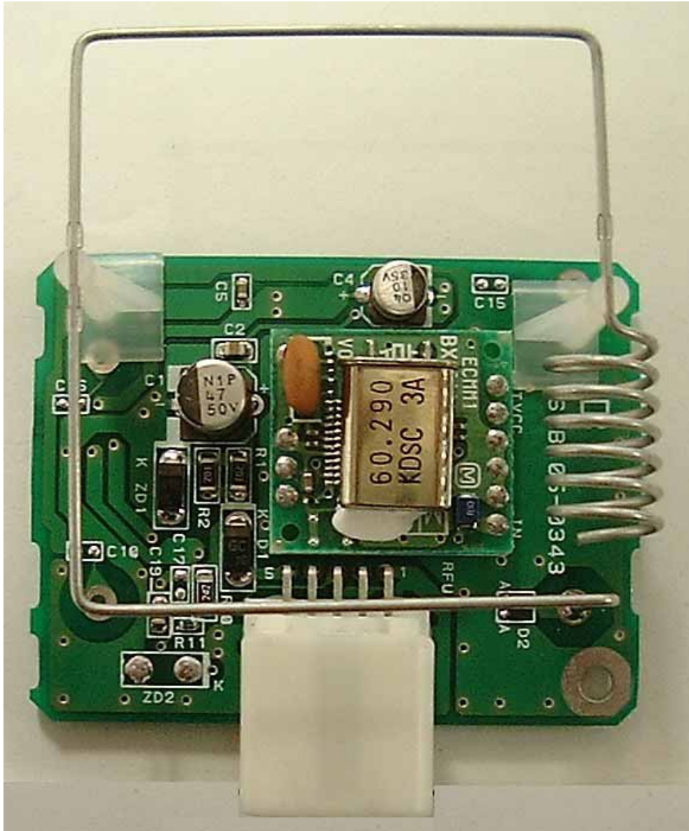
Receiver MDL B21RG Mother Board (Top view)
