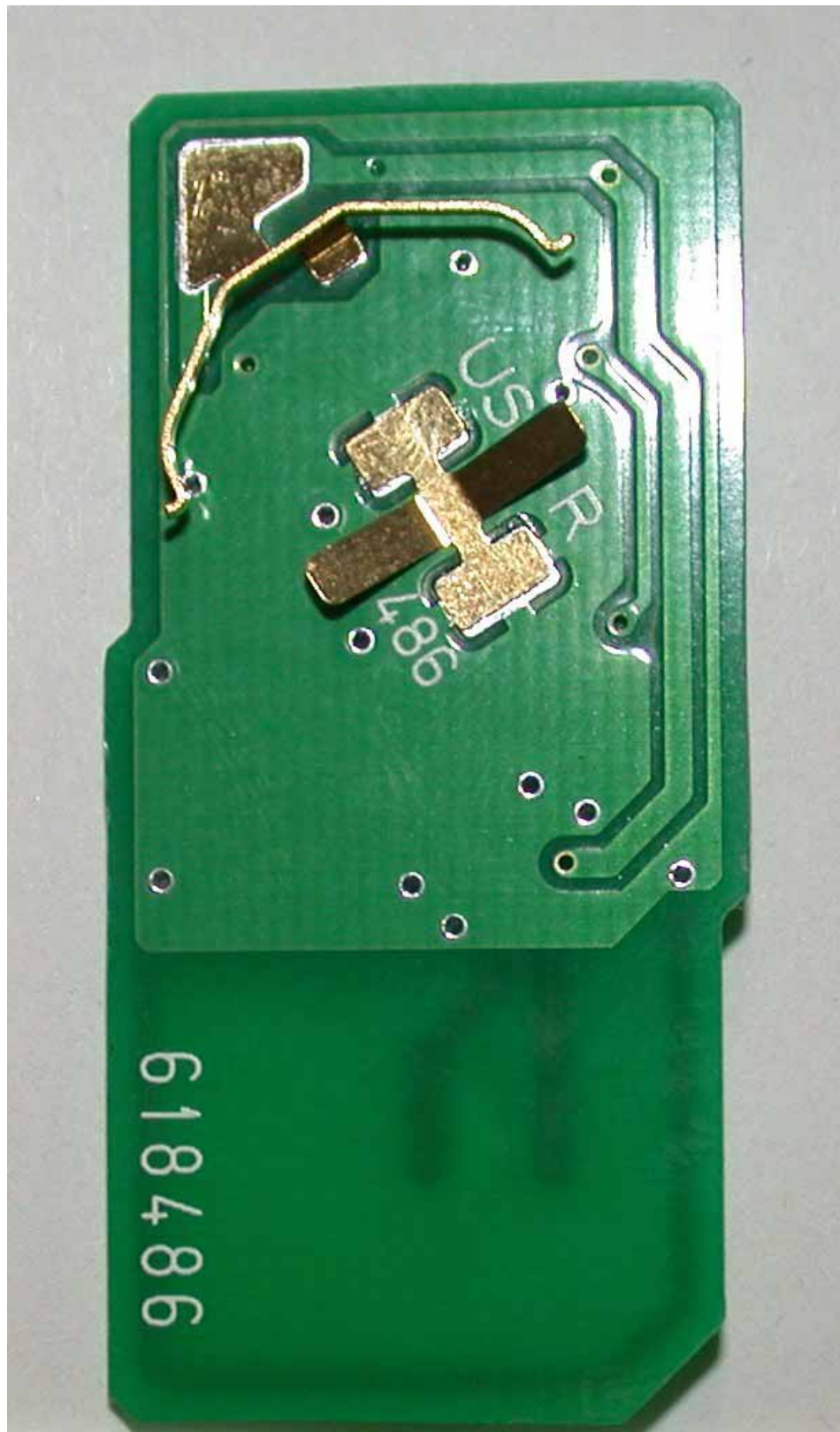
Amplifier MDL B21TG Printed Circuit Board (Bottom view)
