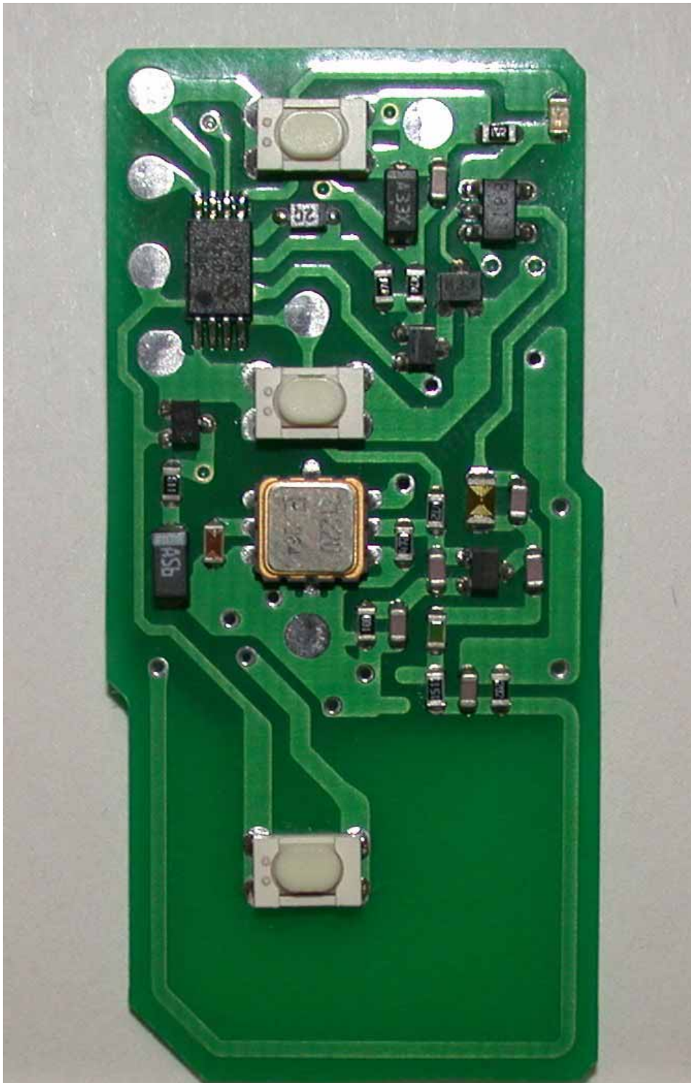
Card Key MDL B21TG Printed Circuit Board (Top view)
