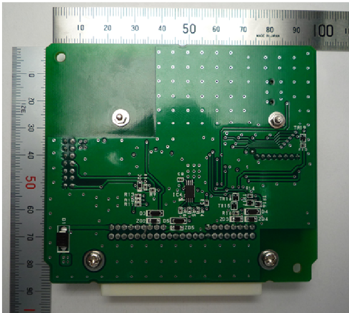
Reverse View
