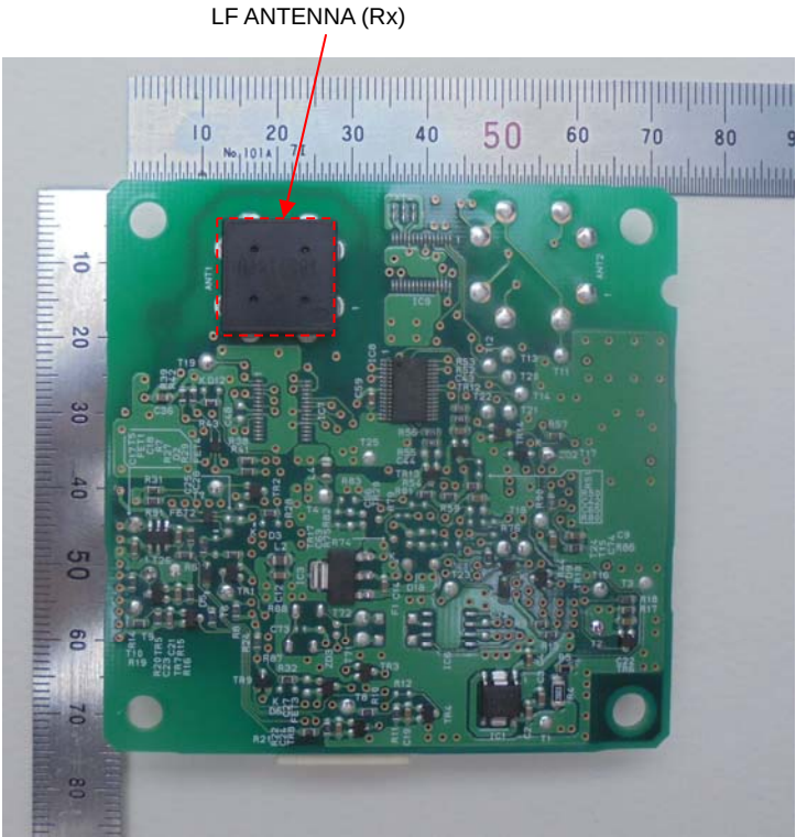
Reverse View
