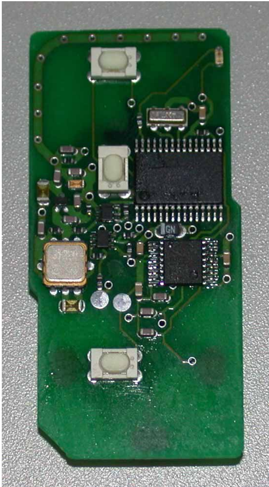
Electronic Key MDL B31EG Printed Circuit Board (Top view)
