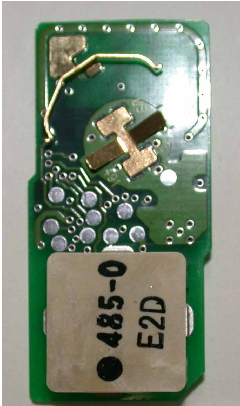
Electronic Key MDL B31EG Printed Circuit Board (Bottom view)
