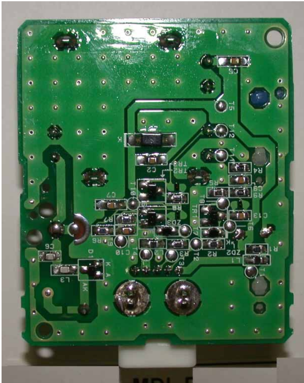
Tuner MDL B31UG Mother Board (Reverse face)
