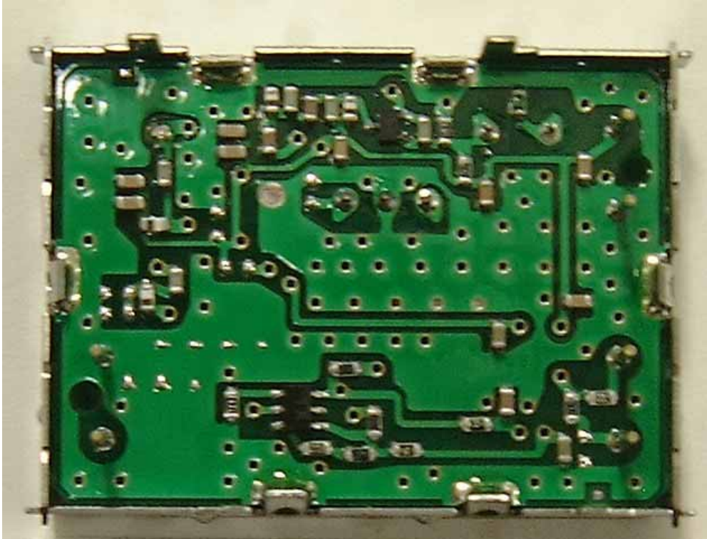
Tuner MDL B31UG RF Module (Reverse face)
