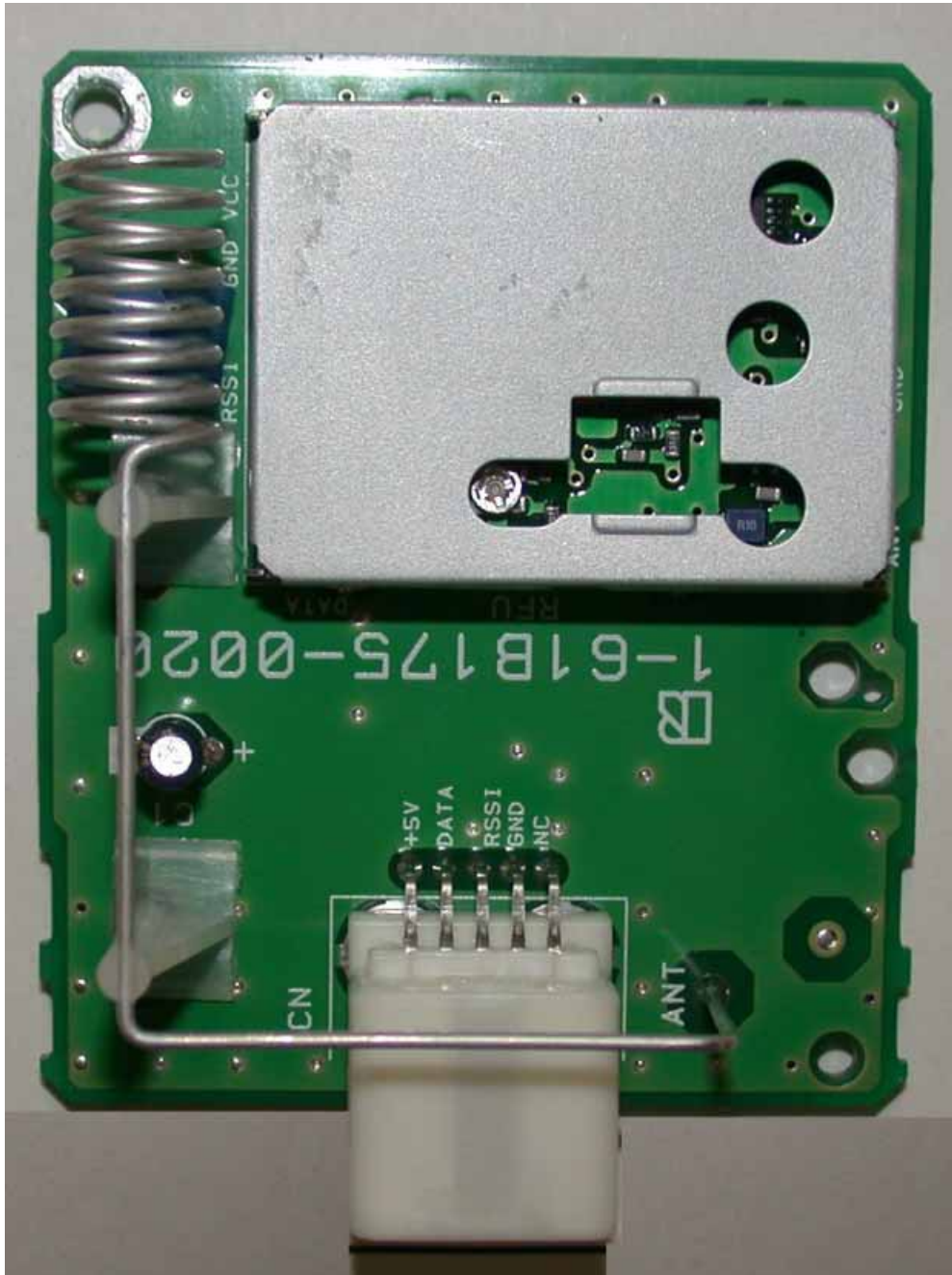
Tuner MDL B31UG Mother Board (Front face)
