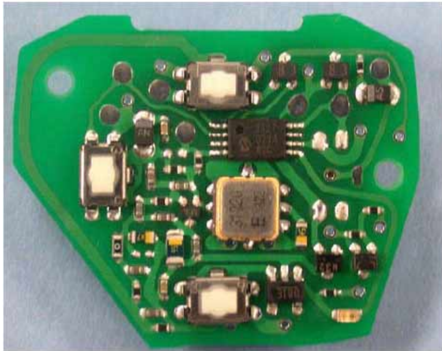
RKE Transmitter MDL B41TG Printed Circuit Board (Front)
