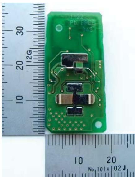
PC board (Rear View)
