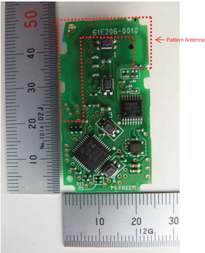
Front View
