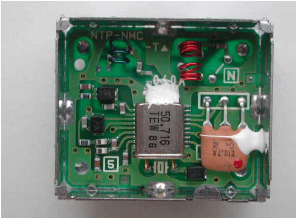
Receiver Module PART No. D02MB
