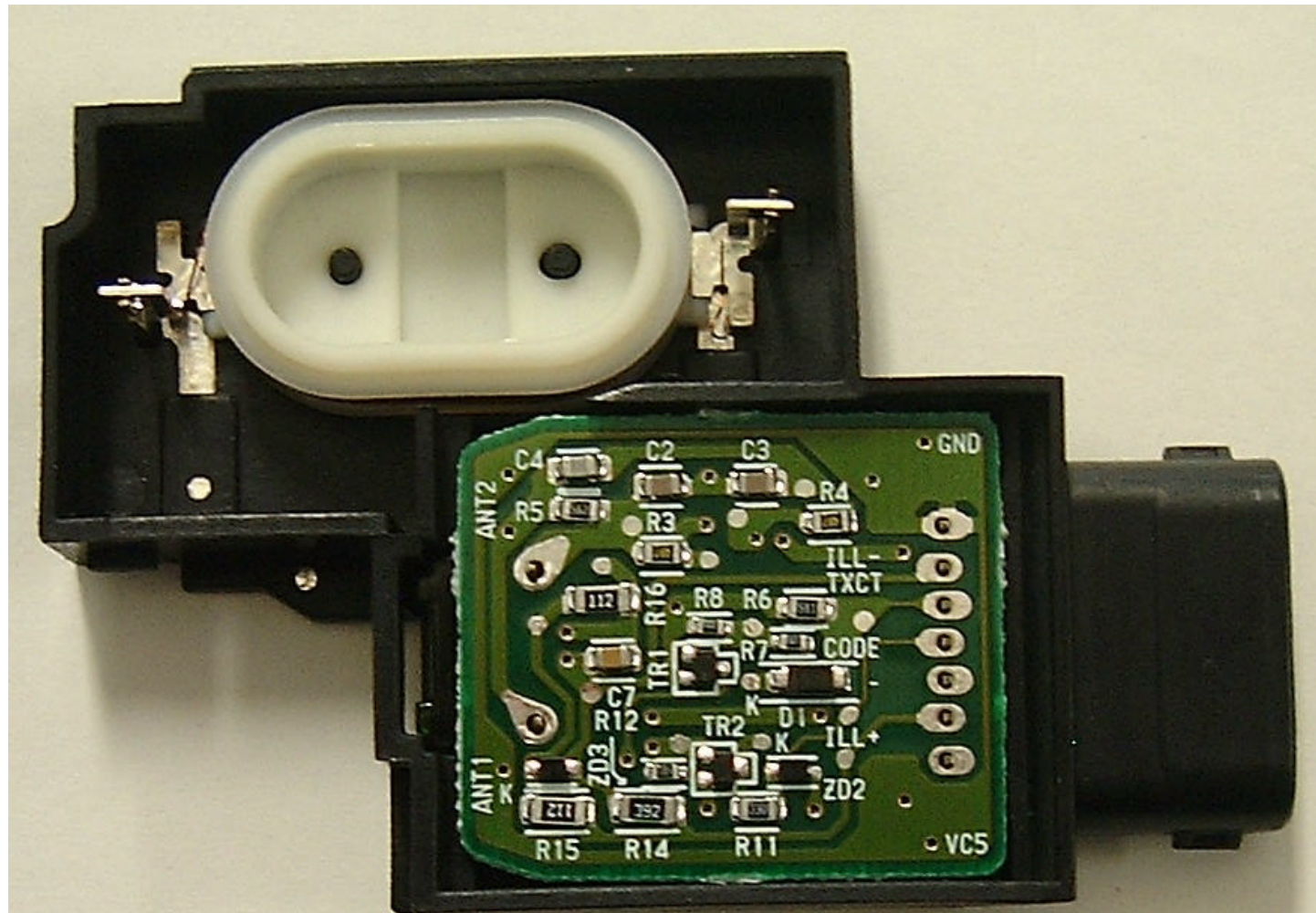
Amplifier MDL RI-24KTY Amplifying Circuit & Coil antenna
