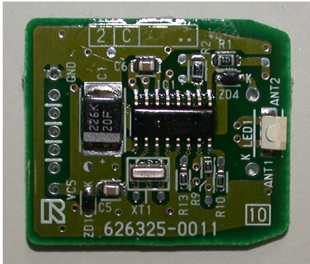
Amplifier MDL RI-24KTY Amplifying Circuit (Top view)
